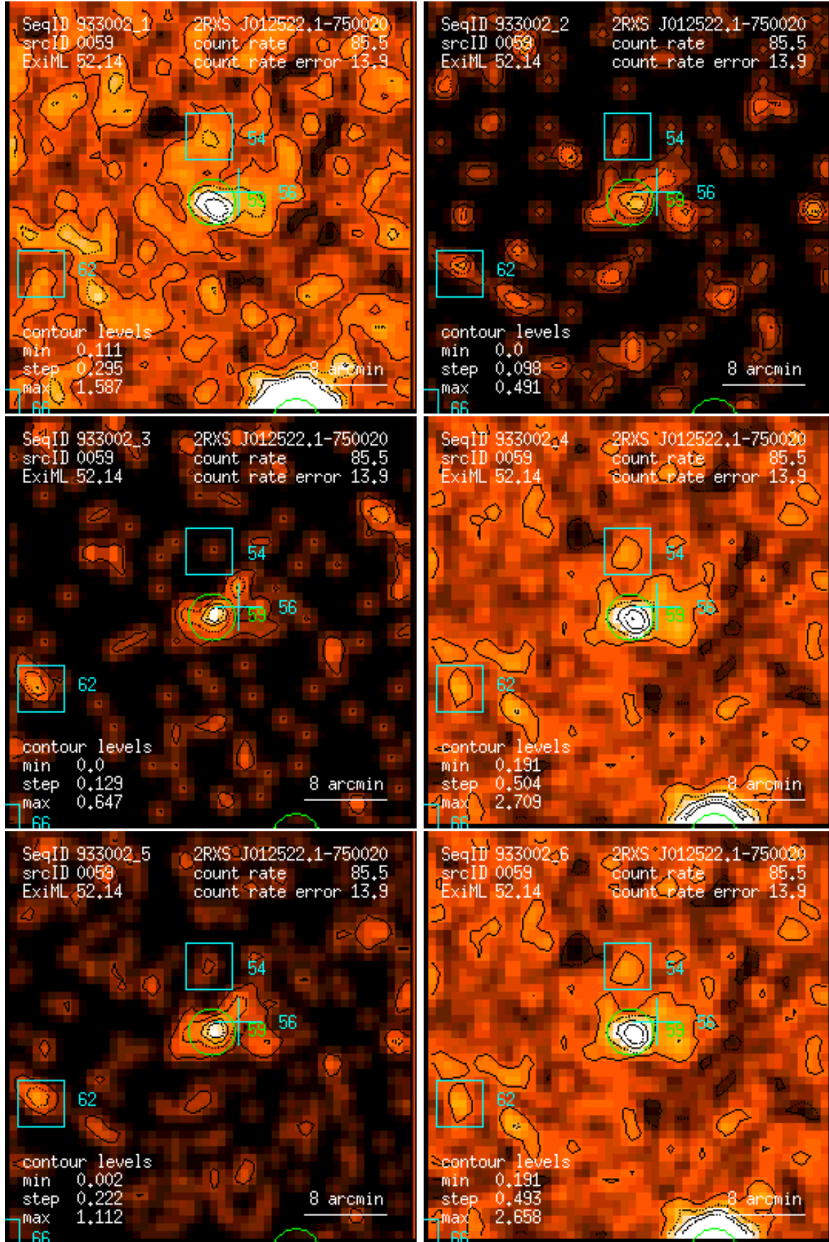
Figure 59: RASS 933002: detection 0059: band rate images, Gaussian filter: (1) PSPC channels 11 – 41, (2) 52 – 90, (3) 91 – 201, (4) 11 – 235, (5) 52 – 201, (6) 11 – 201. Broad band rates in counts/ks. Band rate contour levels in counts/ks/arcmin 2 .
