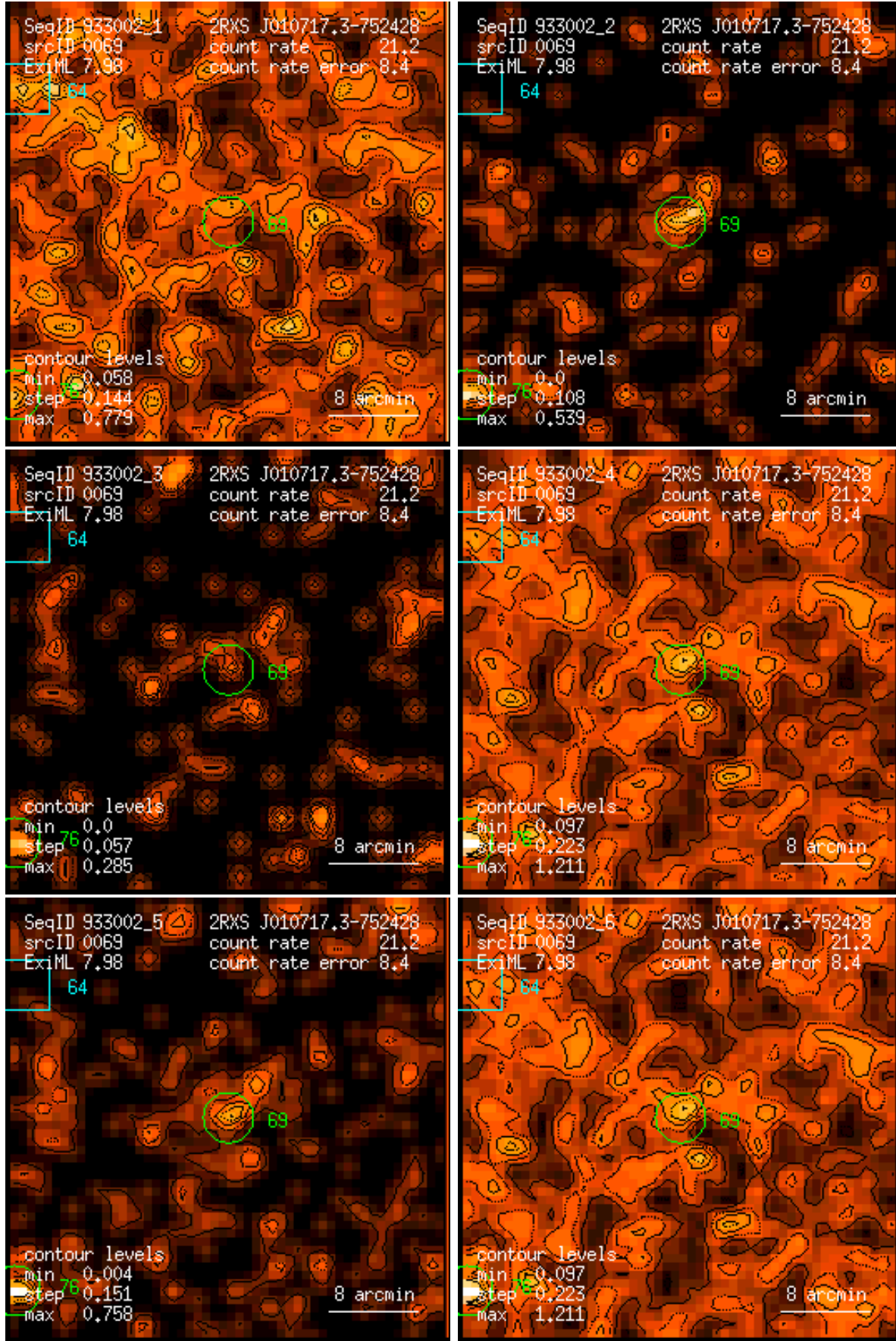
Figure 69: RASS 933002: detection 0069: band rate images, Gaussian filter: (1) PSPC channels 11 – 41, (2) 52 – 90, (3) 91 – 201, (4) 11 – 235, (5) 52 – 201, (6) 11 – 201. Broad band rates in counts/ks. Band rate contour levels in counts/ks/arcmin 2 .
