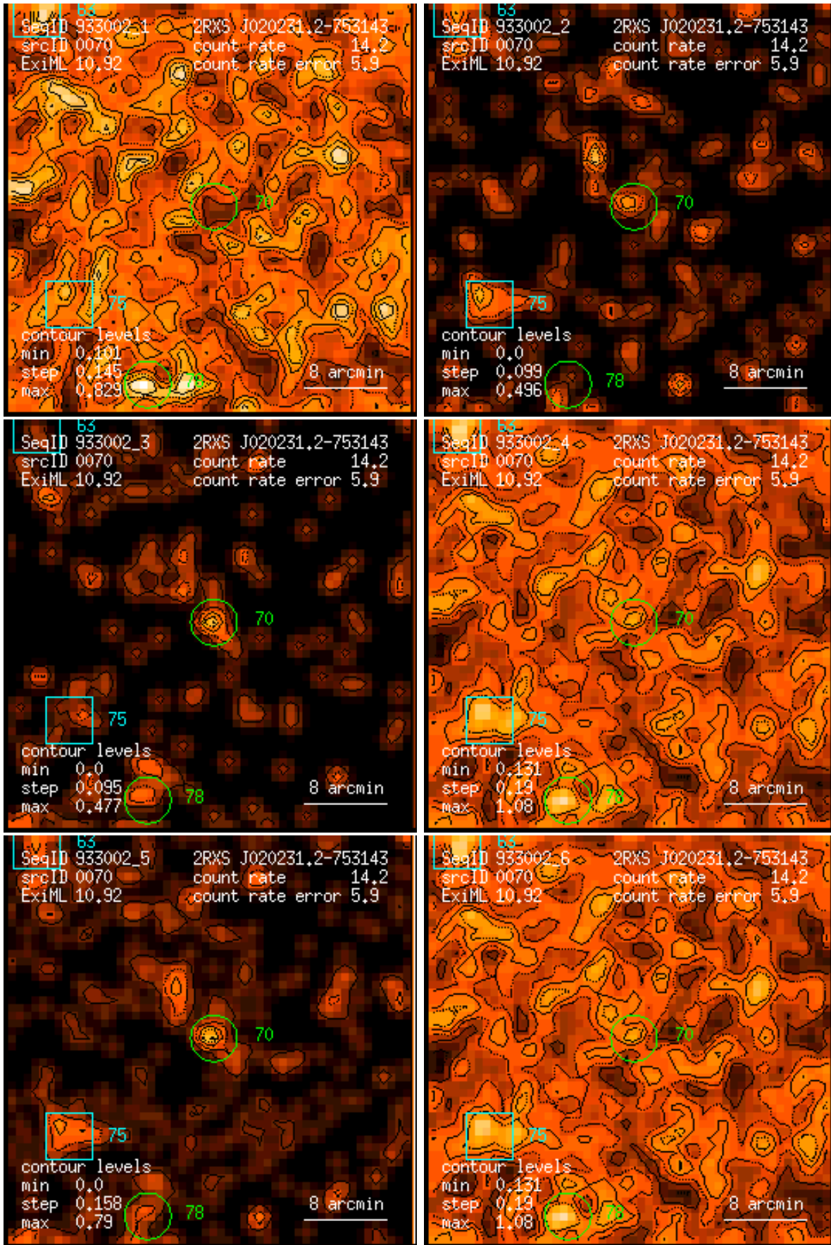
Figure 70: RASS 933002: detection 0070: band rate images, Gaussian filter: (1) PSPC channels 11 – 41, (2) 52 – 90, (3) 91 – 201, (4) 11 – 235, (5) 52 – 201, (6) 11 – 201. Broad band rates in counts/ks. Band rate contour levels in counts/ks/arcmin 2 .
