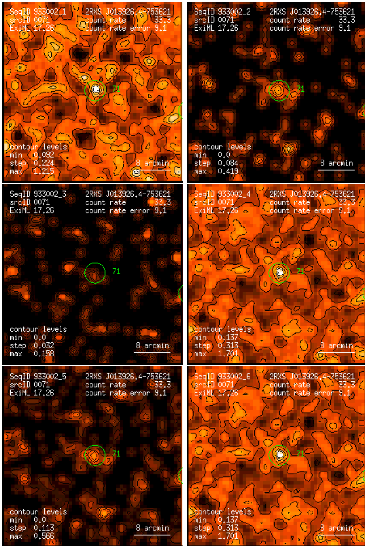
Figure 71: RASS 933002: detection 0071: band rate images, Gaussian filter: (1) PSPC channels 11 – 41, (2) 52 – 90, (3) 91 – 201, (4) 11 – 235, (5) 52 – 201, (6) 11 – 201. Broad band rates in counts/ks. Band rate contour levels in counts/ks/arcmin 2 .
