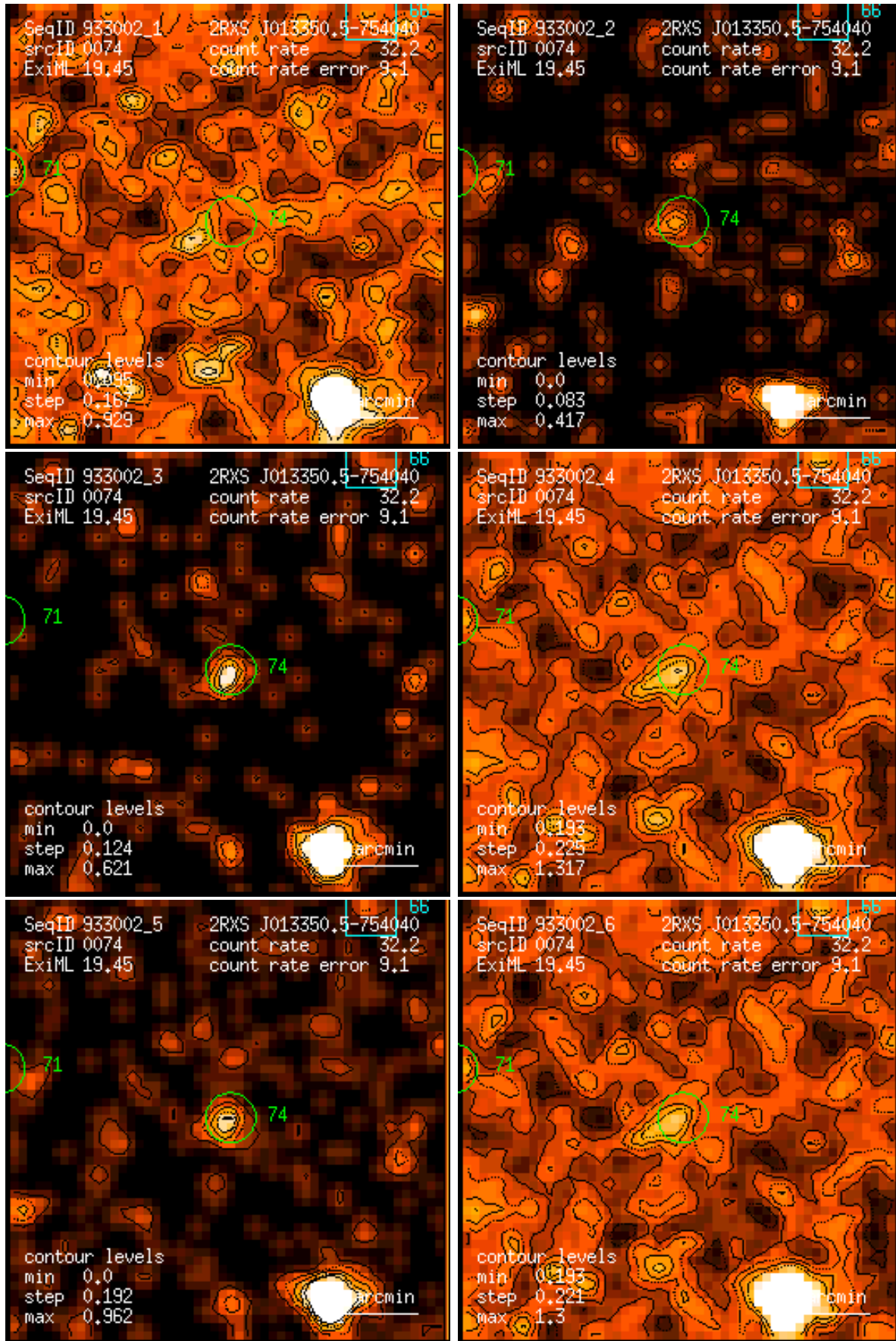
Figure 74: RASS 933002: detection 0074: band rate images, Gaussian filter: (1) PSPC channels 11 – 41, (2) 52 – 90, (3) 91 – 201, (4) 11 – 235, (5) 52 – 201, (6) 11 – 201. Broad band rates in counts/ks. Band rate contour levels in counts/ks/arcmin 2 .
