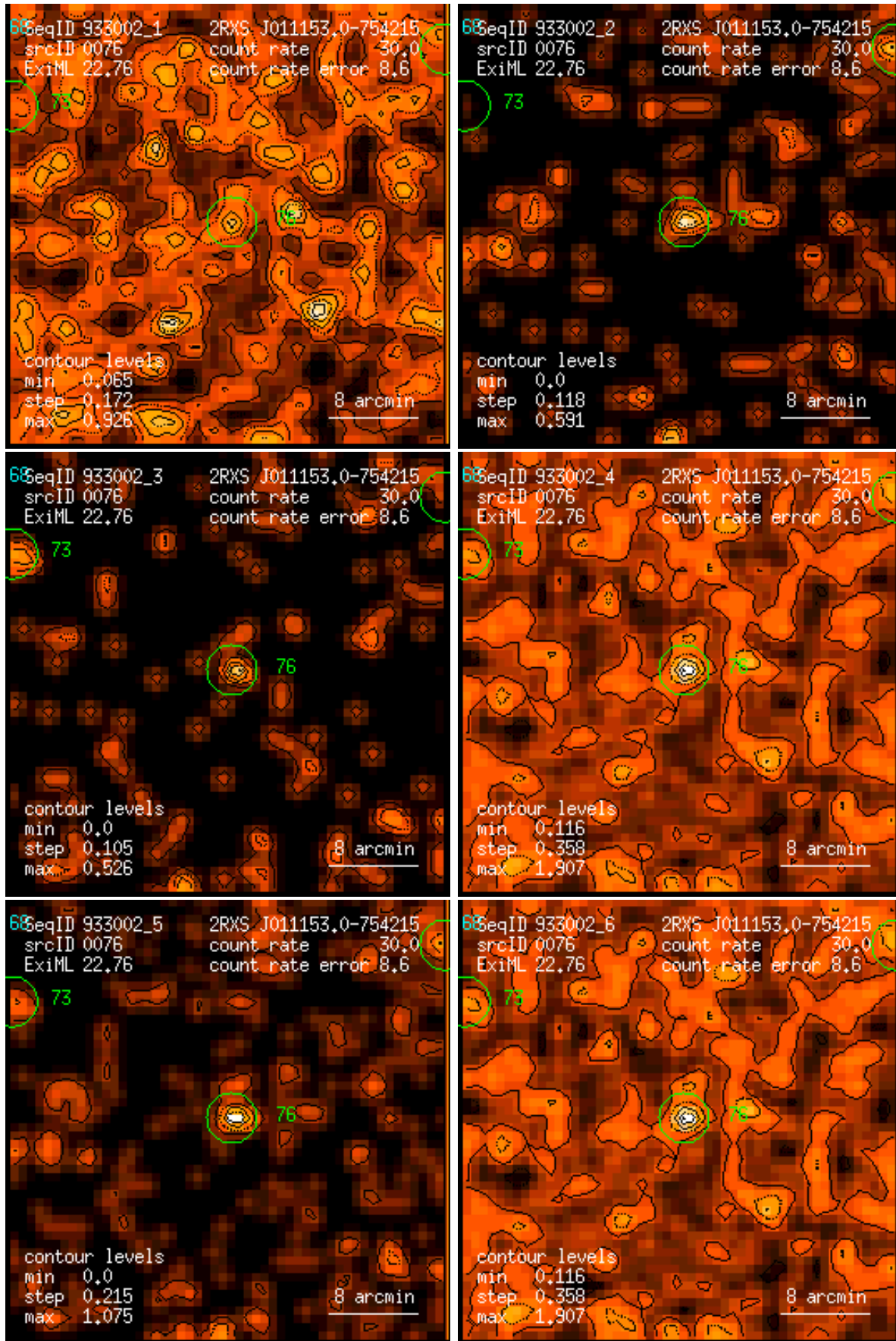
Figure 76: RASS 933002: detection 0076: band rate images, Gaussian filter: (1) PSPC channels 11 – 41, (2) 52 – 90, (3) 91 – 201, (4) 11 – 235, (5) 52 – 201, (6) 11 – 201. Broad band rates in counts/ks. Band rate contour levels in counts/ks/arcmin 2 .
