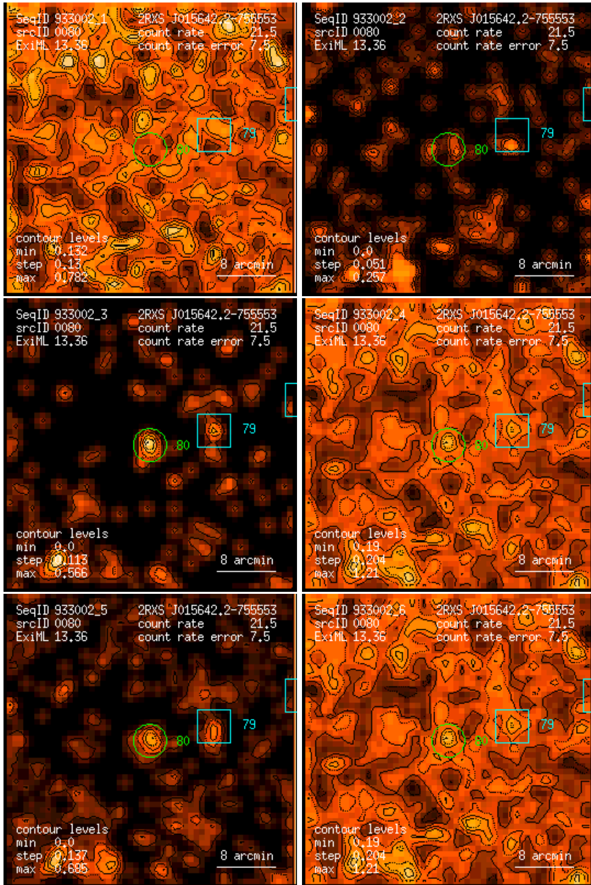
Figure 80: RASS 933002: detection 0080: band rate images, Gaussian filter: (1) PSPC channels 11 – 41, (2) 52 – 90, (3) 91 – 201, (4) 11 – 235, (5) 52 – 201, (6) 11 – 201. Broad band rates in counts/ks. Band rate contour levels in counts/ks/arcmin 2 .
