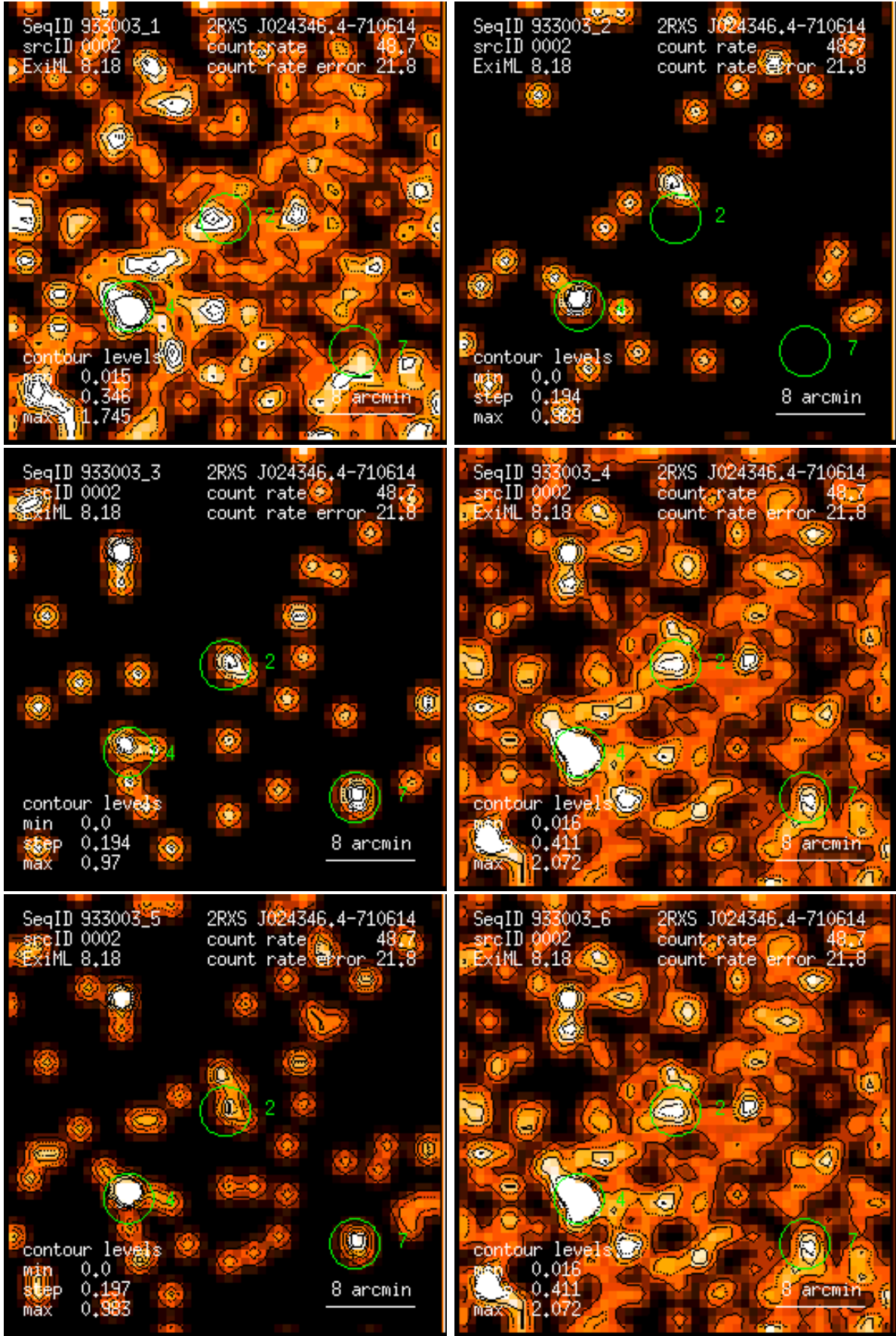
Figure 2: RASS 933003: detection 0002: band rate images, Gaussian filter: (1) PSPC channels 11 – 41, (2) 52 – 90, (3) 91 – 201, (4) 11 – 235, (5) 52 – 201, (6) 11 – 201. Broad band rates in counts/ks. Band rate contour levels in counts/ks/arcmin 2 .
