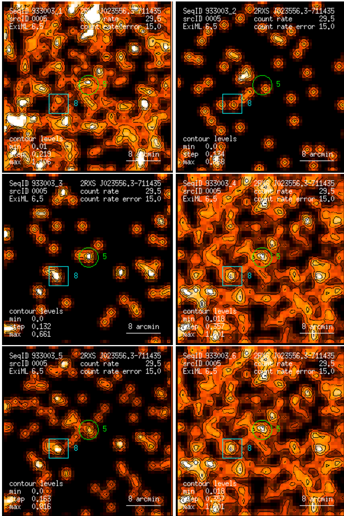
Figure 5: RASS 933003: detection 0005: band rate images, Gaussian filter: (1) PSPC channels 11 – 41, (2) 52 – 90, (3) 91 – 201, (4) 11 – 235, (5) 52 – 201, (6) 11 – 201. Broad band rates in counts/ks. Band rate contour levels in counts/ks/arcmin 2 .
