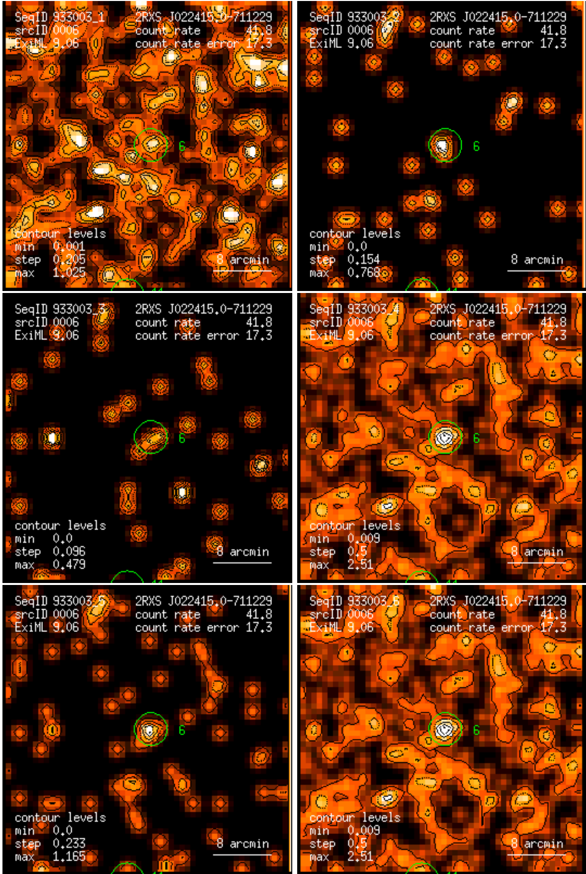
Figure 6: RASS 933003: detection 0006: band rate images, Gaussian filter: (1) PSPC channels 11 – 41, (2) 52 – 90, (3) 91 – 201, (4) 11 – 235, (5) 52 – 201, (6) 11 – 201. Broad band rates in counts/ks. Band rate contour levels in counts/ks/arcmin 2 .
