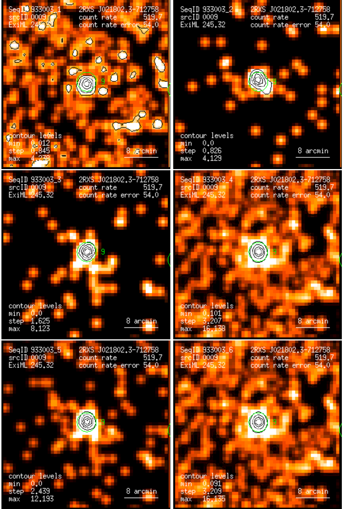
Figure 9: RASS 933003: detection 0009: band rate images, Gaussian filter: (1) PSPC channels 11 – 41, (2) 52 – 90, (3) 91 – 201, (4) 11 – 235, (5) 52 – 201, (6) 11 – 201. Broad band rates in counts/ks. Band rate contour levels in counts/ks/arcmin 2 .
