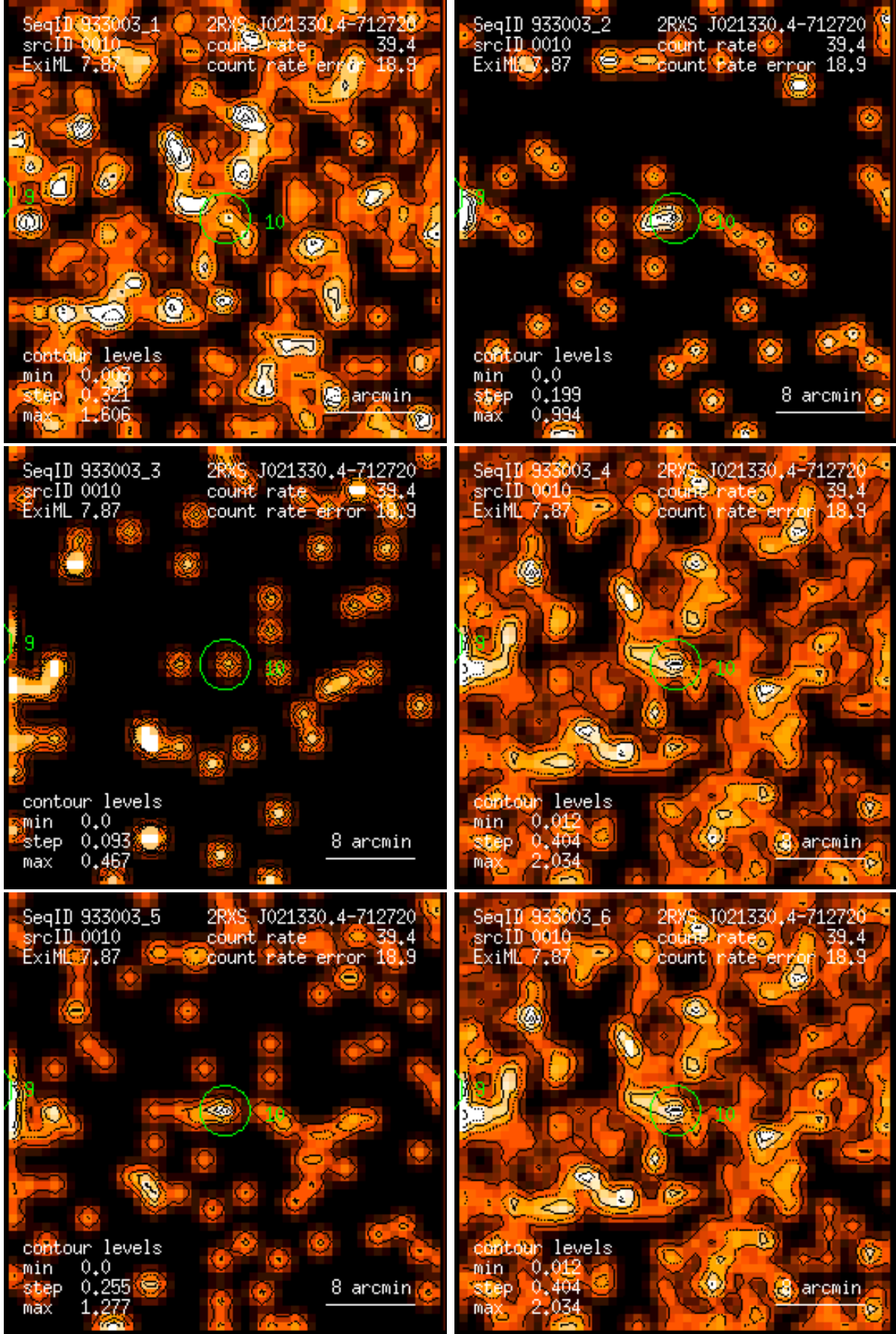
Figure 10: RASS 933003: detection 0010: band rate images, Gaussian filter: (1) PSPC channels 11 – 41, (2) 52 – 90, (3) 91 – 201, (4) 11 – 235, (5) 52 – 201, (6) 11 – 201. Broad band rates in counts/ks. Band rate contour levels in counts/ks/arcmin 2 .
