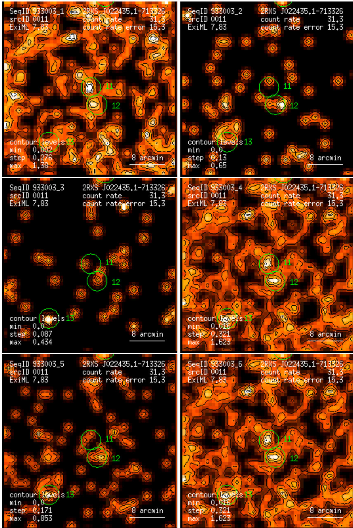
Figure 11: RASS 933003: detection 0011: band rate images, Gaussian filter: (1) PSPC channels 11 – 41, (2) 52 – 90, (3) 91 – 201, (4) 11 – 235, (5) 52 – 201, (6) 11 – 201. Broad band rates in counts/ks. Band rate contour levels in counts/ks/arcmin 2 .
