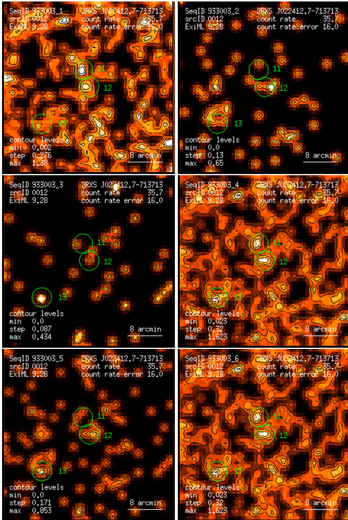
Figure 12: RASS 933003: detection 0012: band rate images, Gaussian filter: (1) PSPC channels 11 – 41, (2) 52 – 90, (3) 91 – 201, (4) 11 – 235, (5) 52 – 201, (6) 11 – 201. Broad band rates in counts/ks. Band rate contour levels in counts/ks/arcmin 2 .
