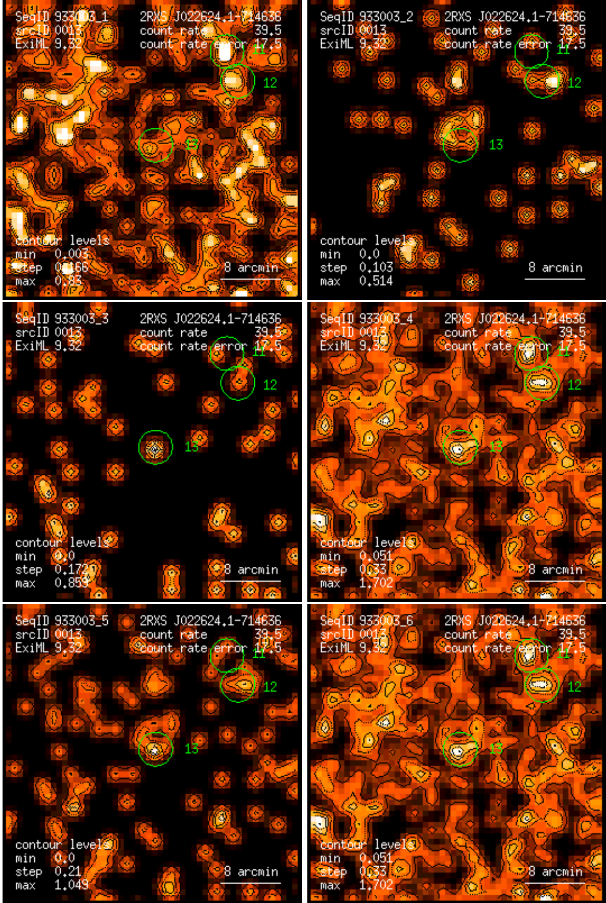
Figure 13: RASS 933003: detection 0013: band rate images, Gaussian filter: (1) PSPC channels 11 – 41, (2) 52 – 90, (3) 91 – 201, (4) 11 – 235, (5) 52 – 201, (6) 11 – 201. Broad band rates in counts/ks. Band rate contour levels in counts/ks/arcmin 2 .
