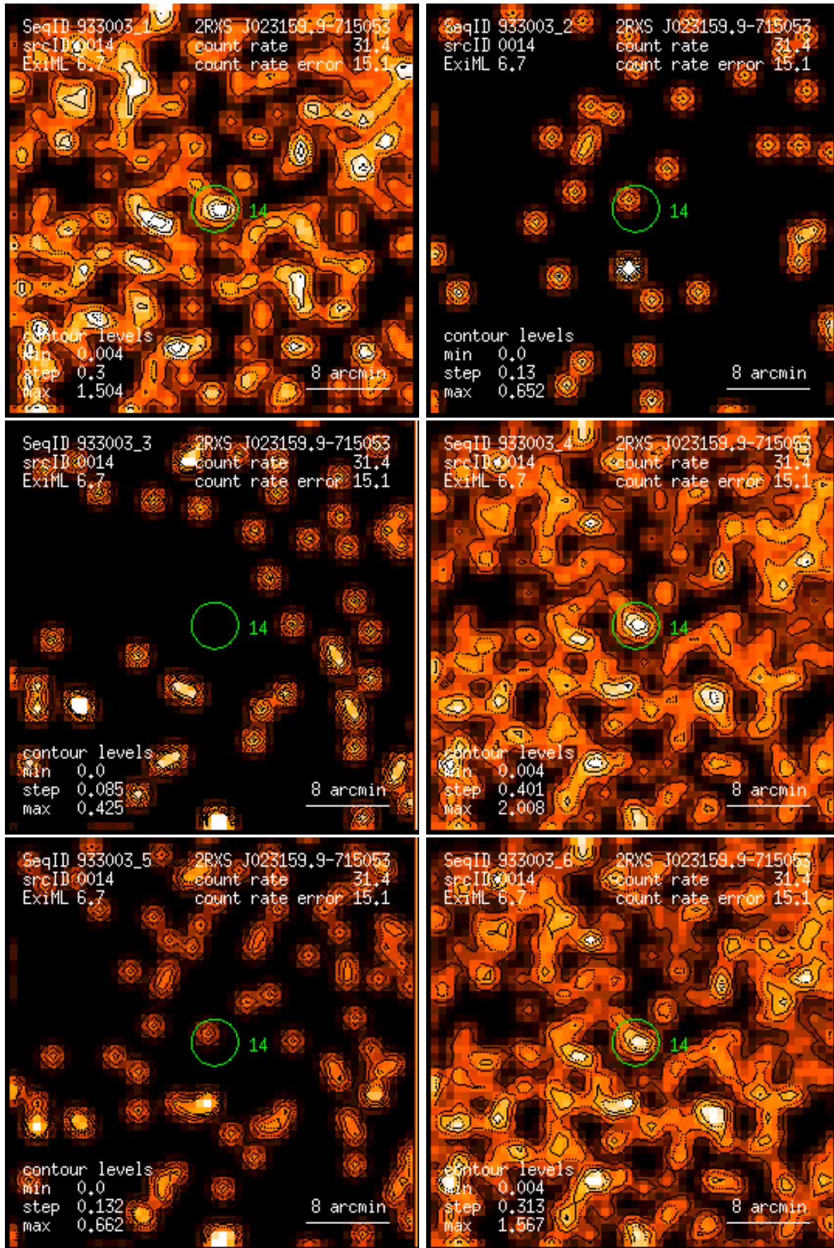
Figure 14: RASS 933003: detection 0014: band rate images, Gaussian filter: (1) PSPC channels 11 – 41, (2) 52 – 90, (3) 91 – 201, (4) 11 – 235, (5) 52 – 201, (6) 11 – 201. Broad band rates in counts/ks. Band rate contour levels in counts/ks/arcmin 2 .
