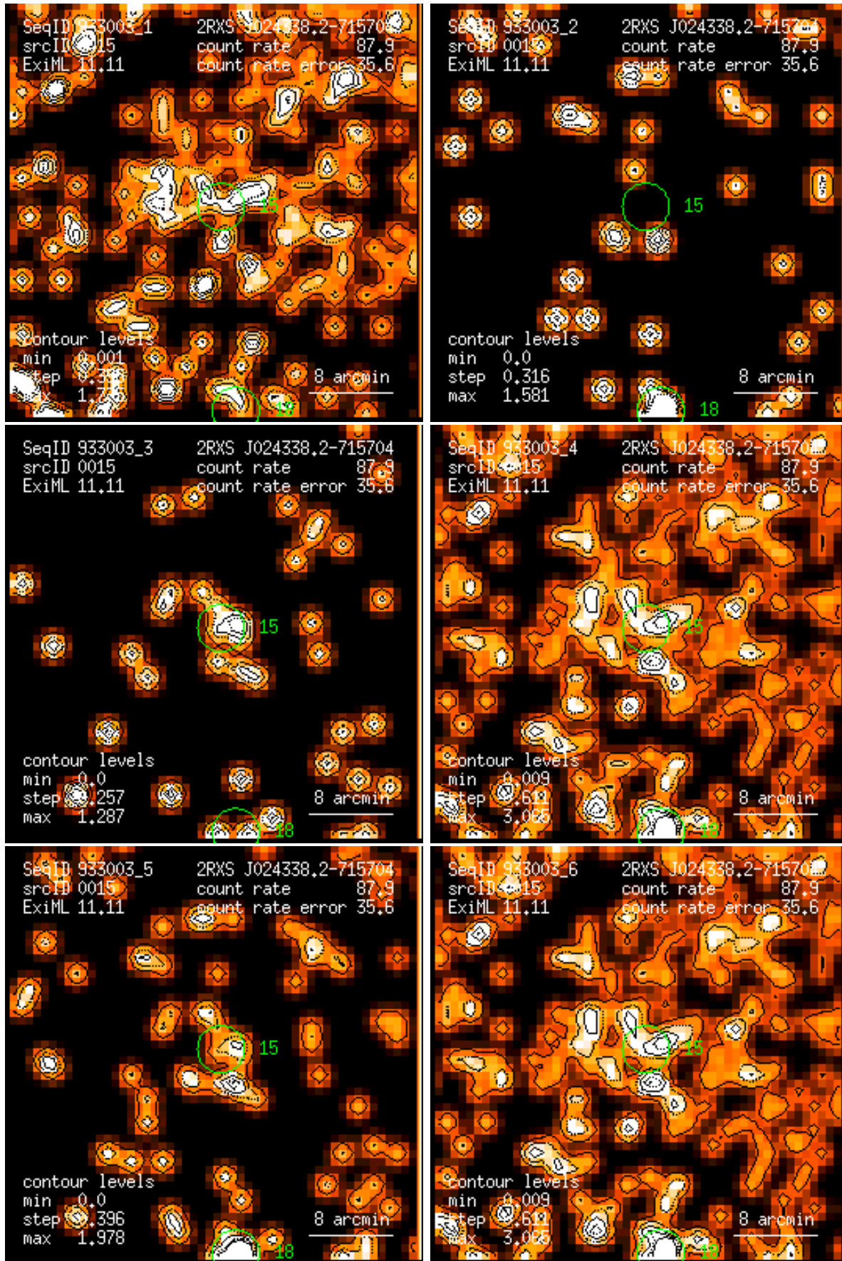
Figure 15: RASS 933003: detection 0015: band rate images, Gaussian filter: (1) PSPC channels 11 – 41, (2) 52 – 90, (3) 91 – 201, (4) 11 – 235, (5) 52 – 201, (6) 11 – 201. Broad band rates in counts/ks. Band rate contour levels in counts/ks/arcmin 2 .
