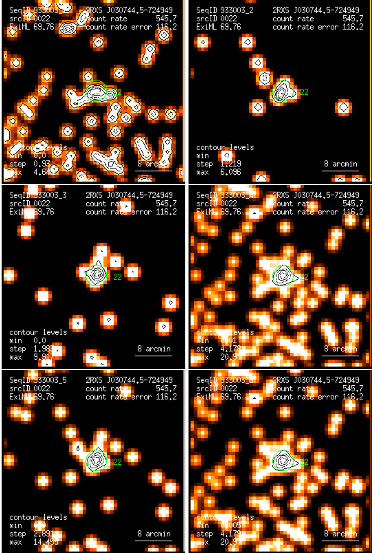
Figure 22: RASS 933003: detection 0022: band rate images, Gaussian filter: (1) PSPC channels 11 – 41, (2) 52 – 90, (3) 91 – 201, (4) 11 – 235, (5) 52 – 201, (6) 11 – 201. Broad band rates in counts/ks. Band rate contour levels in counts/ks/arcmin 2 .
