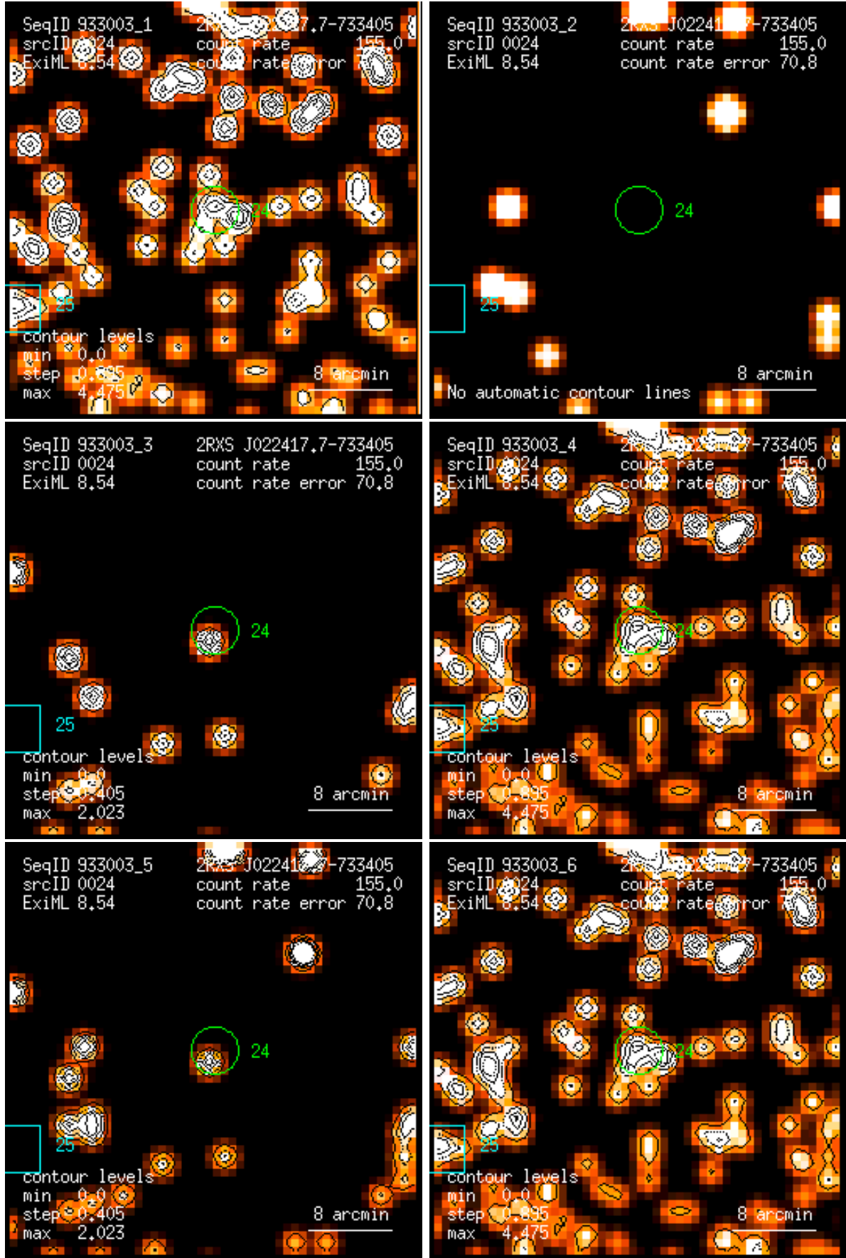
Figure 24: RASS 933003: detection 0024: band rate images, Gaussian filter: (1) PSPC channels 11 – 41, (2) 52 – 90, (3) 91 – 201, (4) 11 – 235, (5) 52 – 201, (6) 11 – 201. Broad band rates in counts/ks. Band rate contour levels in counts/ks/arcmin 2 .
