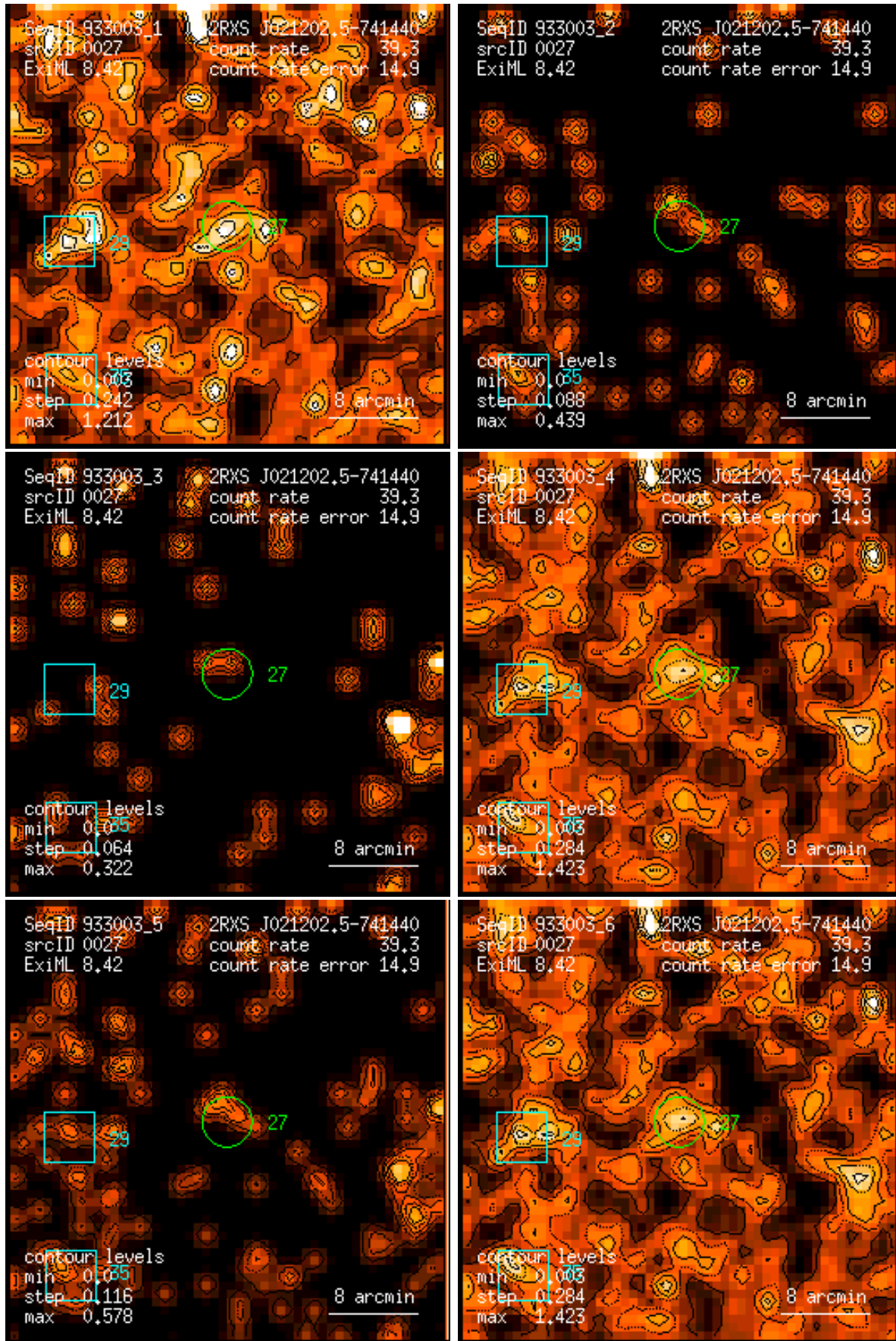
Figure 27: RASS 933003: detection 0027: band rate images, Gaussian filter: (1) PSPC channels 11 – 41, (2) 52 – 90, (3) 91 – 201, (4) 11 – 235, (5) 52 – 201, (6) 11 – 201. Broad band rates in counts/ks. Band rate contour levels in counts/ks/arcmin 2 .
