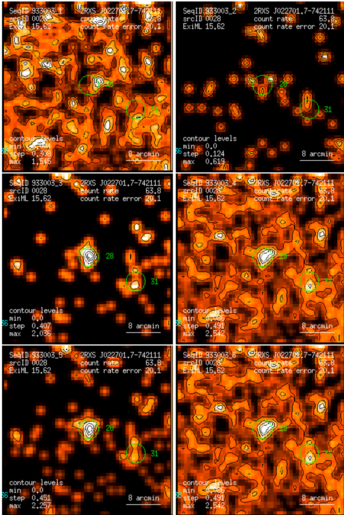
Figure 28: RASS 933003: detection 0028: band rate images, Gaussian filter: (1) PSPC channels 11 – 41, (2) 52 – 90, (3) 91 – 201, (4) 11 – 235, (5) 52 – 201, (6) 11 – 201. Broad band rates in counts/ks. Band rate contour levels in counts/ks/arcmin 2 .
