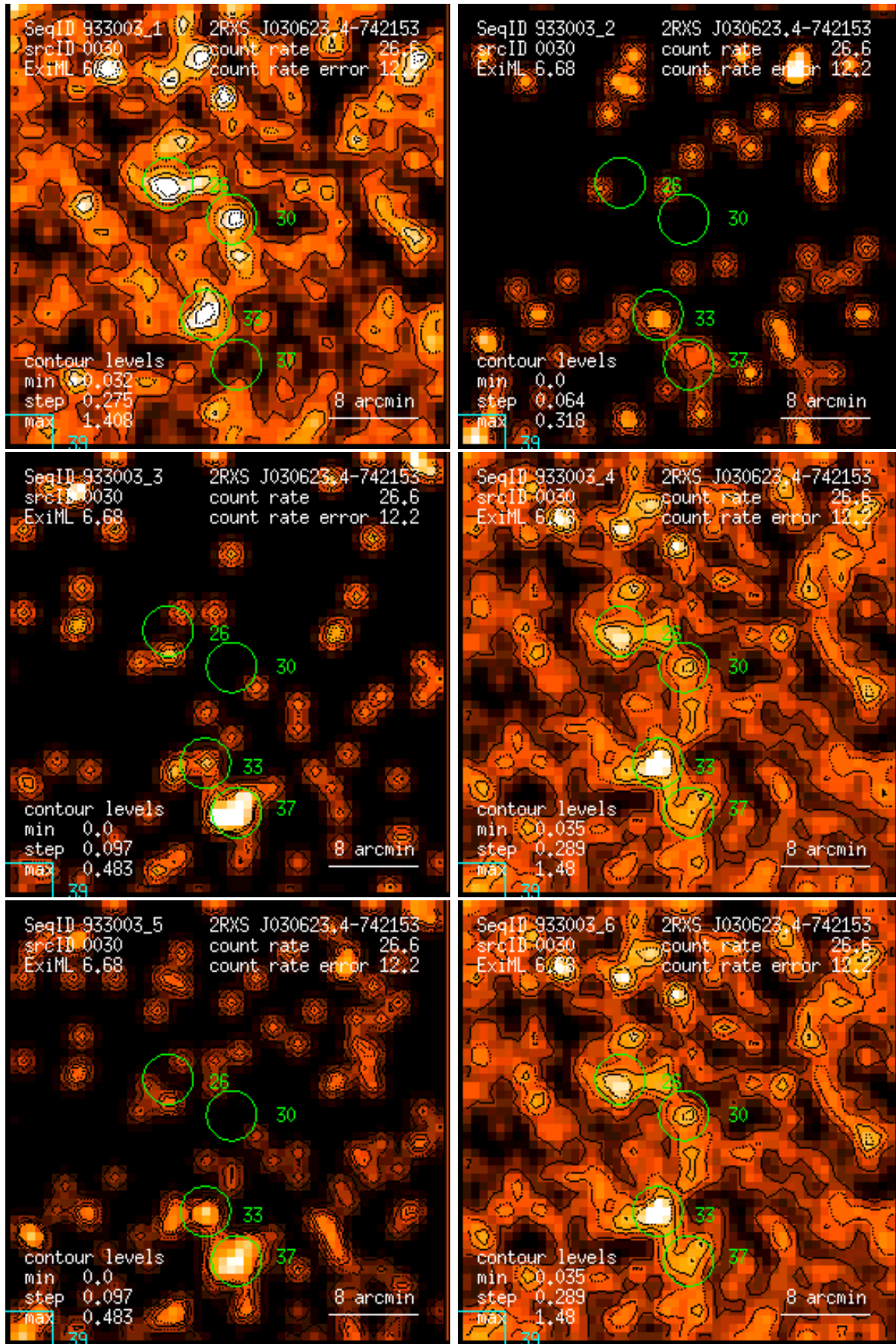
Figure 30: RASS 933003: detection 0030: band rate images, Gaussian filter: (1) PSPC channels 11 – 41, (2) 52 – 90, (3) 91 – 201, (4) 11 – 235, (5) 52 – 201, (6) 11 – 201. Broad band rates in counts/ks. Band rate contour levels in counts/ks/arcmin 2 .
