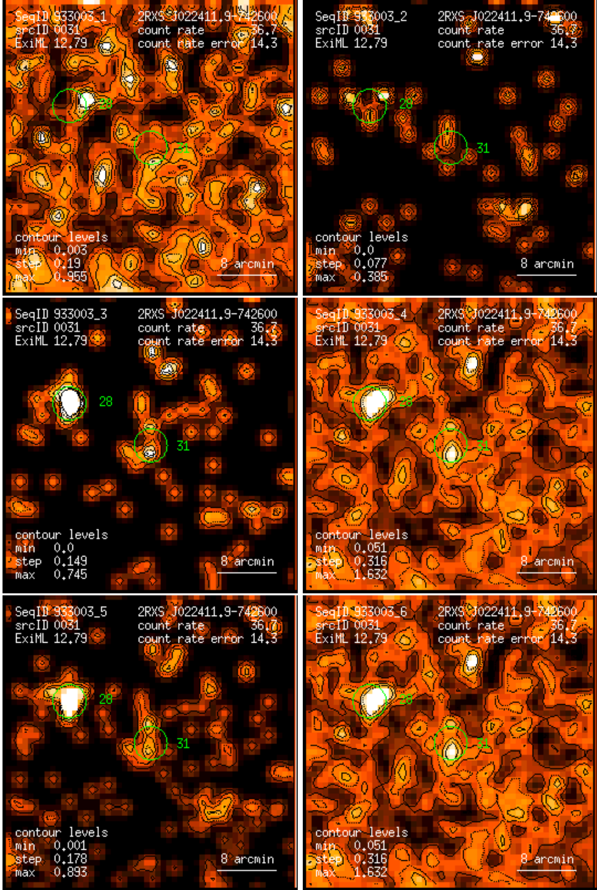
Figure 31: RASS 933003: detection 0031: band rate images, Gaussian filter: (1) PSPC channels 11 – 41, (2) 52 – 90, (3) 91 – 201, (4) 11 – 235, (5) 52 – 201, (6) 11 – 201. Broad band rates in counts/ks. Band rate contour levels in counts/ks/arcmin 2 .
