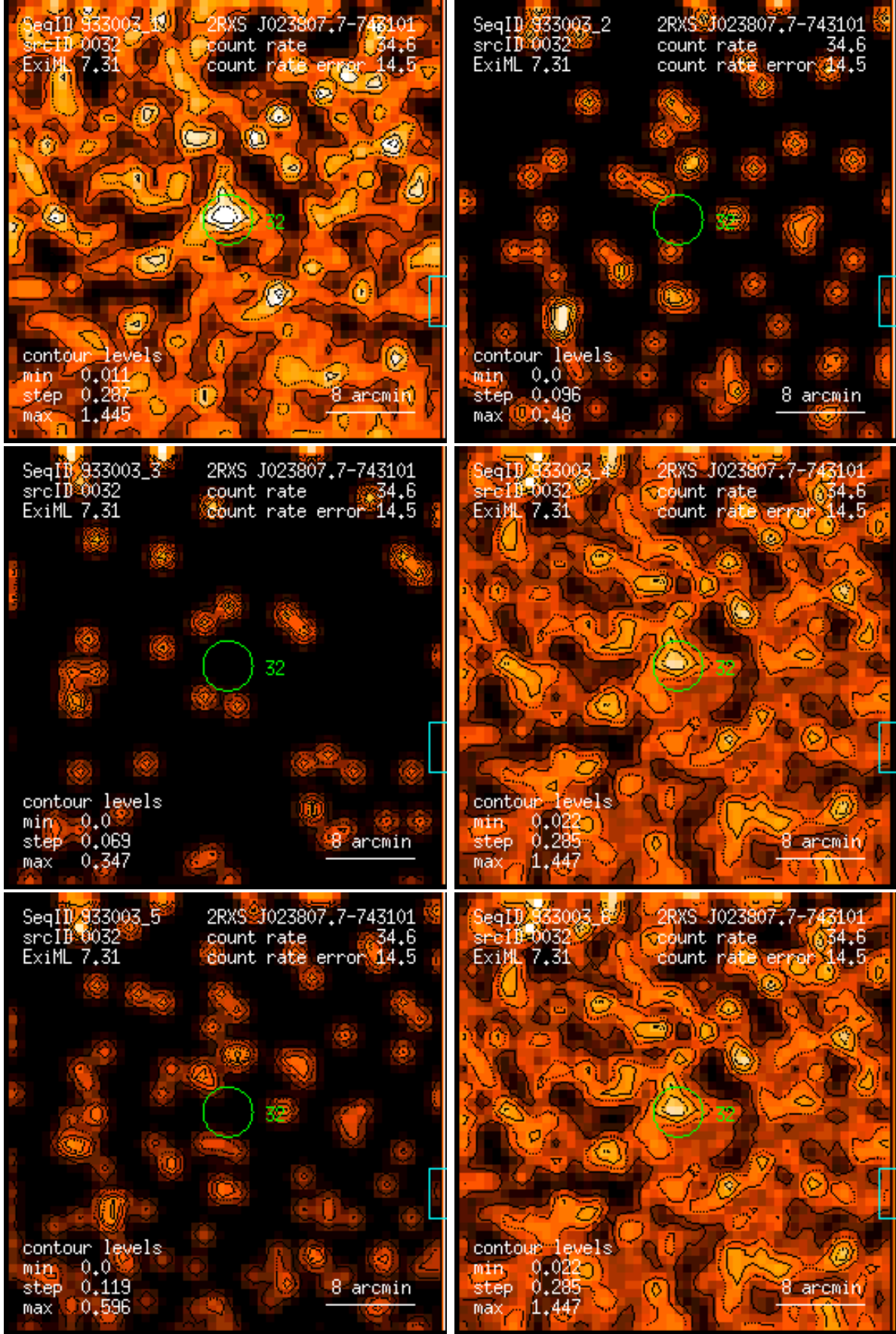
Figure 32: RASS 933003: detection 0032: band rate images, Gaussian filter: (1) PSPC channels 11 – 41, (2) 52 – 90, (3) 91 – 201, (4) 11 – 235, (5) 52 – 201, (6) 11 – 201. Broad band rates in counts/ks. Band rate contour levels in counts/ks/arcmin 2 .
