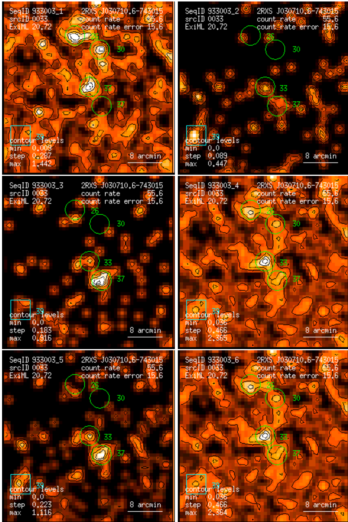
Figure 33: RASS 933003: detection 0033: band rate images, Gaussian filter: (1) PSPC channels 11 – 41, (2) 52 – 90, (3) 91 – 201, (4) 11 – 235, (5) 52 – 201, (6) 11 – 201. Broad band rates in counts/ks. Band rate contour levels in counts/ks/arcmin 2 .
