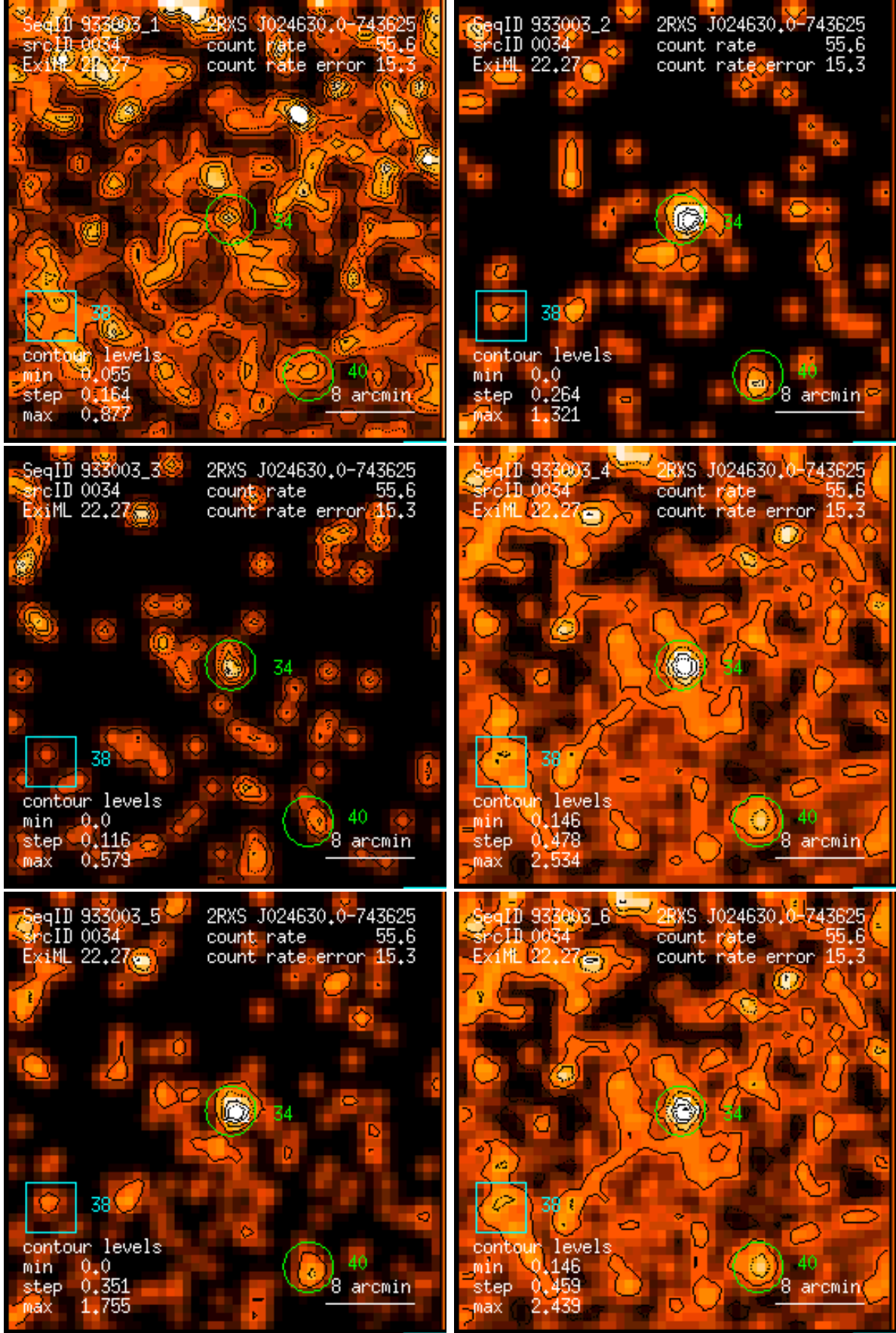
Figure 34: RASS 933003: detection 0034: band rate images, Gaussian filter: (1) PSPC channels 11 – 41, (2) 52 – 90, (3) 91 – 201, (4) 11 – 235, (5) 52 – 201, (6) 11 – 201. Broad band rates in counts/ks. Band rate contour levels in counts/ks/arcmin 2 .
