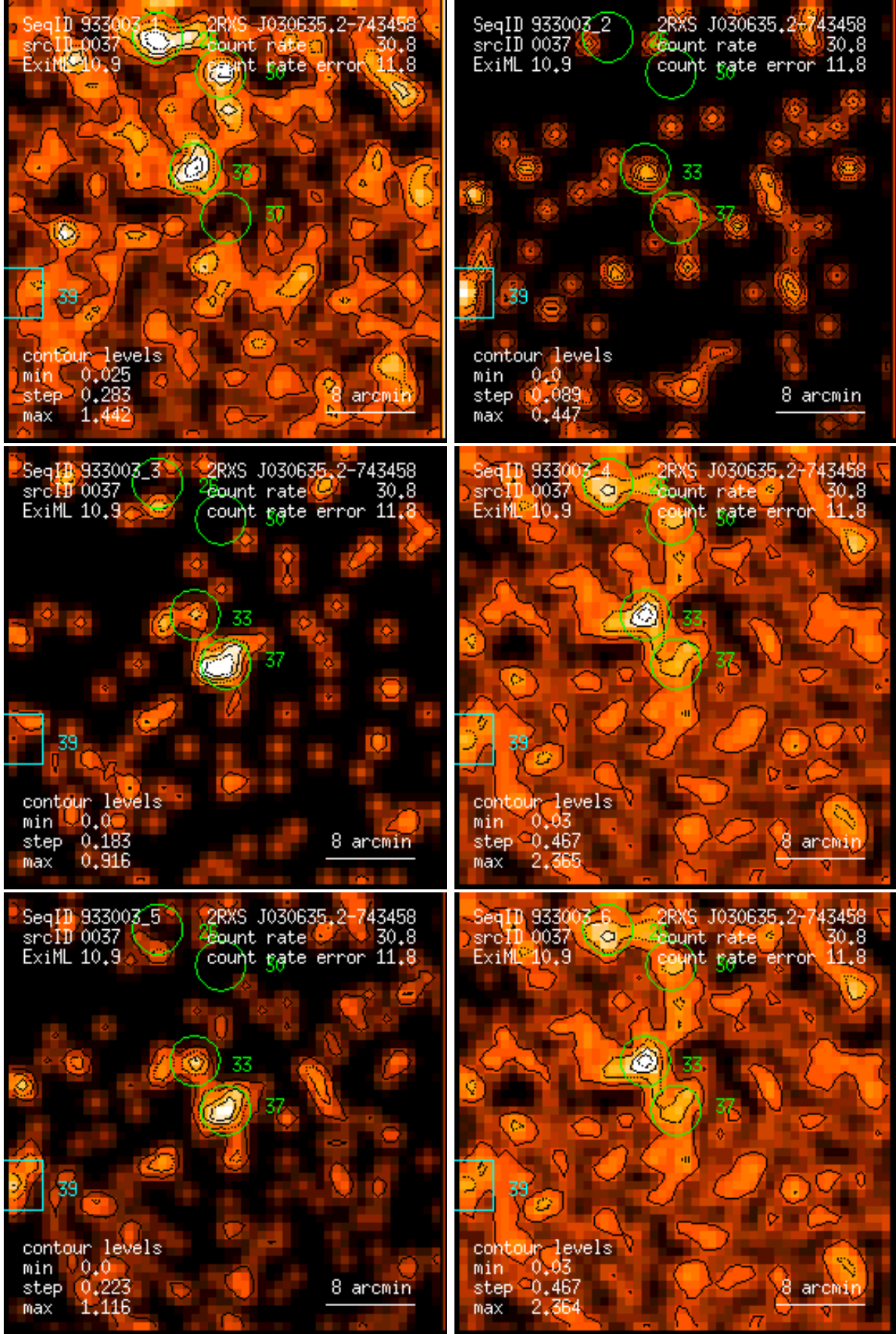
Figure 37: RASS 933003: detection 0037: band rate images, Gaussian filter: (1) PSPC channels 11 – 41, (2) 52 – 90, (3) 91 – 201, (4) 11 – 235, (5) 52 – 201, (6) 11 – 201. Broad band rates in counts/ks. Band rate contour levels in counts/ks/arcmin 2 .
