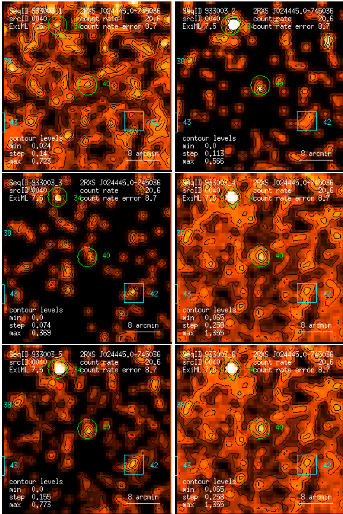
Figure 40: RASS 933003: detection 0040: band rate images, Gaussian filter: (1) PSPC channels 11 – 41, (2) 52 – 90, (3) 91 – 201, (4) 11 – 235, (5) 52 – 201, (6) 11 – 201. Broad band rates in counts/ks. Band rate contour levels in counts/ks/arcmin 2 .
