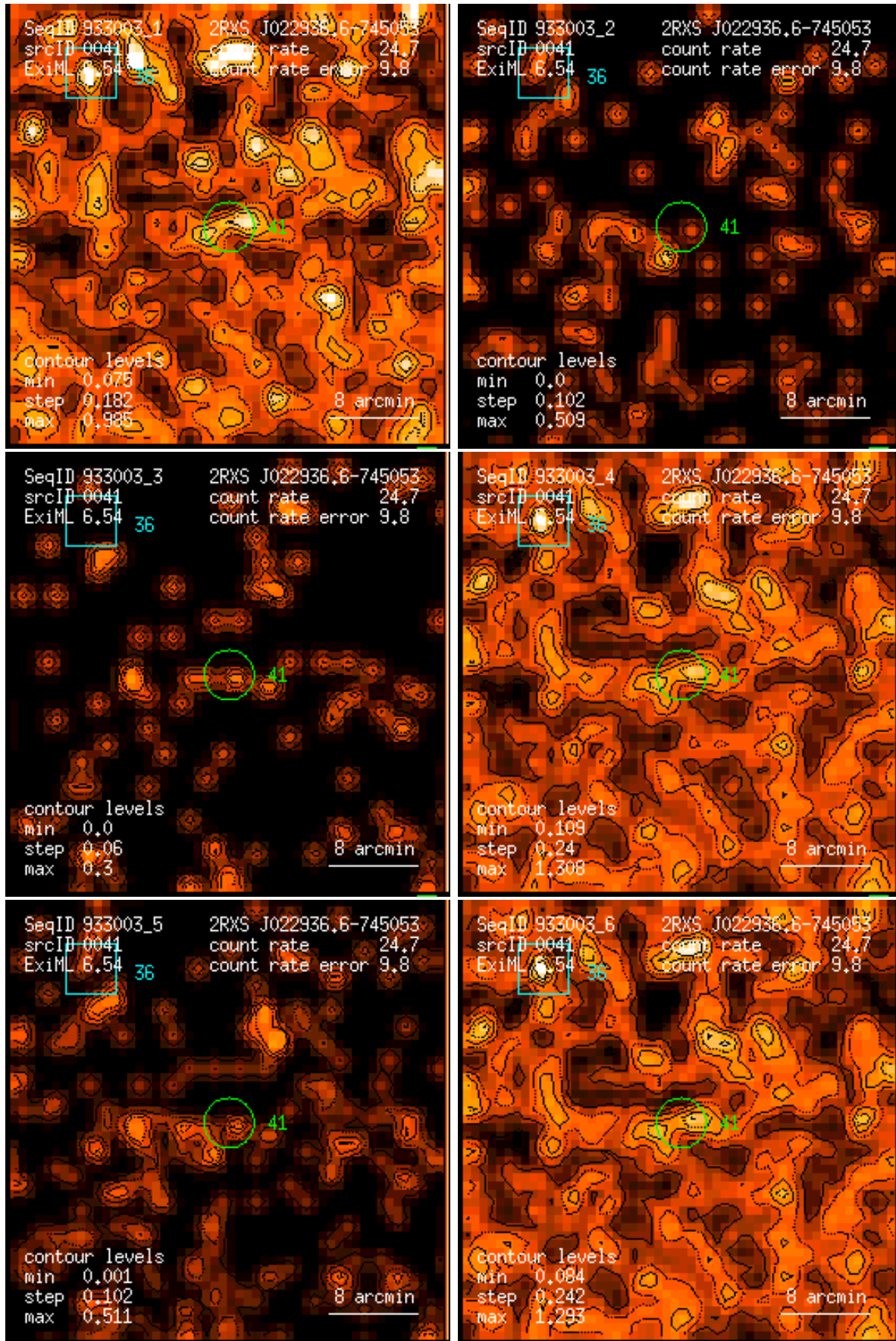
Figure 41: RASS 933003: detection 0041: band rate images, Gaussian filter: (1) PSPC channels 11 – 41, (2) 52 – 90, (3) 91 – 201, (4) 11 – 235, (5) 52 – 201, (6) 11 – 201. Broad band rates in counts/ks. Band rate contour levels in counts/ks/arcmin 2 .
