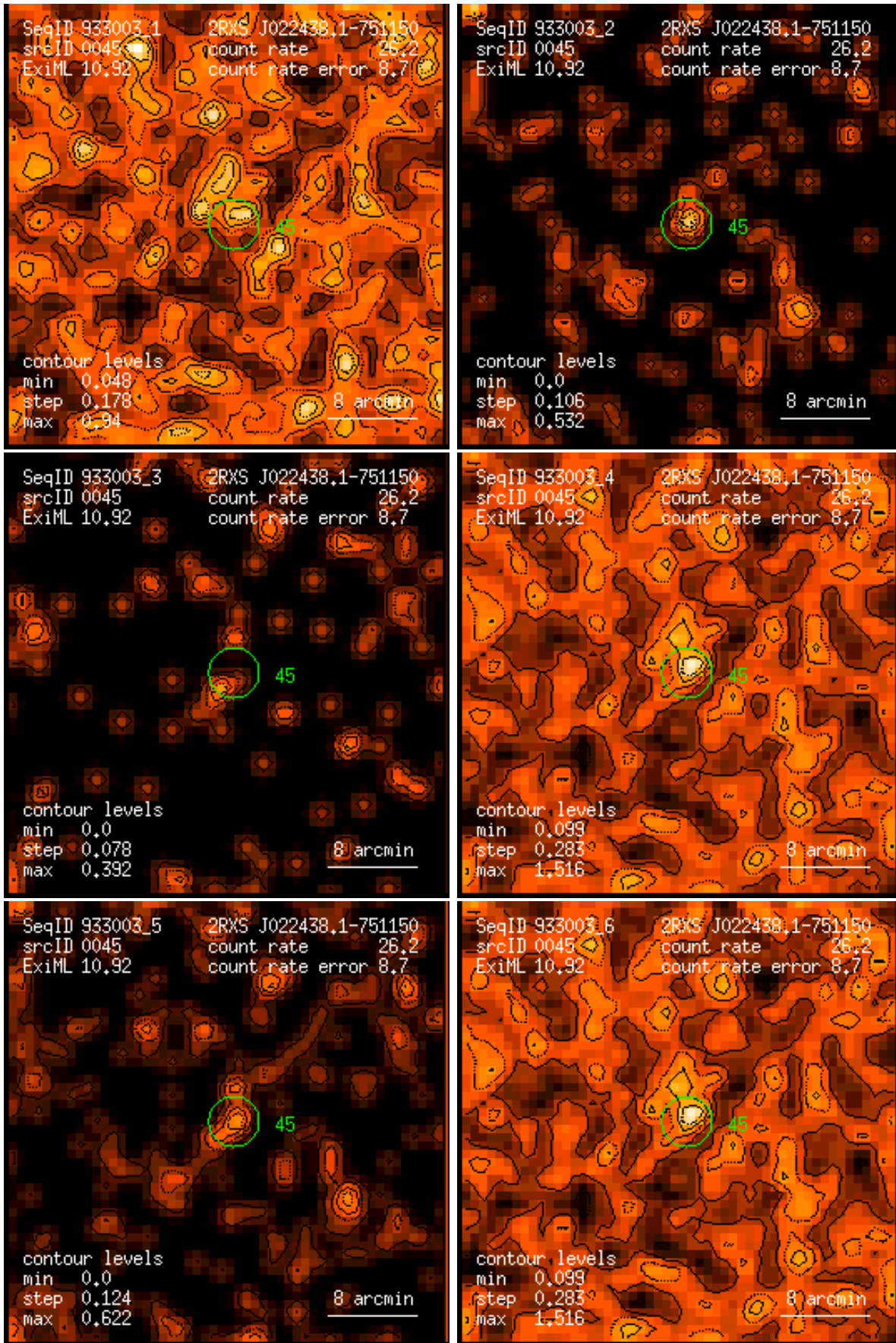
Figure 45: RASS 933003: detection 0045: band rate images, Gaussian filter: (1) PSPC channels 11 – 41, (2) 52 – 90, (3) 91 – 201, (4) 11 – 235, (5) 52 – 201, (6) 11 – 201. Broad band rates in counts/ks. Band rate contour levels in counts/ks/arcmin 2 .
