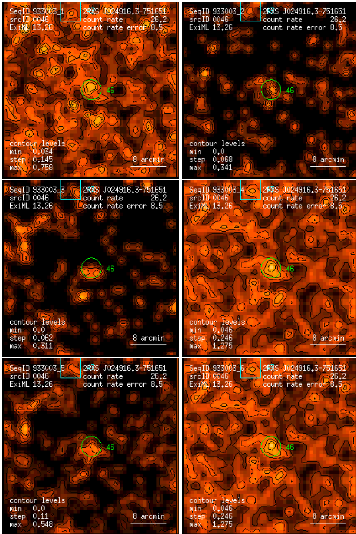
Figure 46: RASS 933003: detection 0046: band rate images, Gaussian filter: (1) PSPC channels 11 – 41, (2) 52 – 90, (3) 91 – 201, (4) 11 – 235, (5) 52 – 201, (6) 11 – 201. Broad band rates in counts/ks. Band rate contour levels in counts/ks/arcmin 2 .
