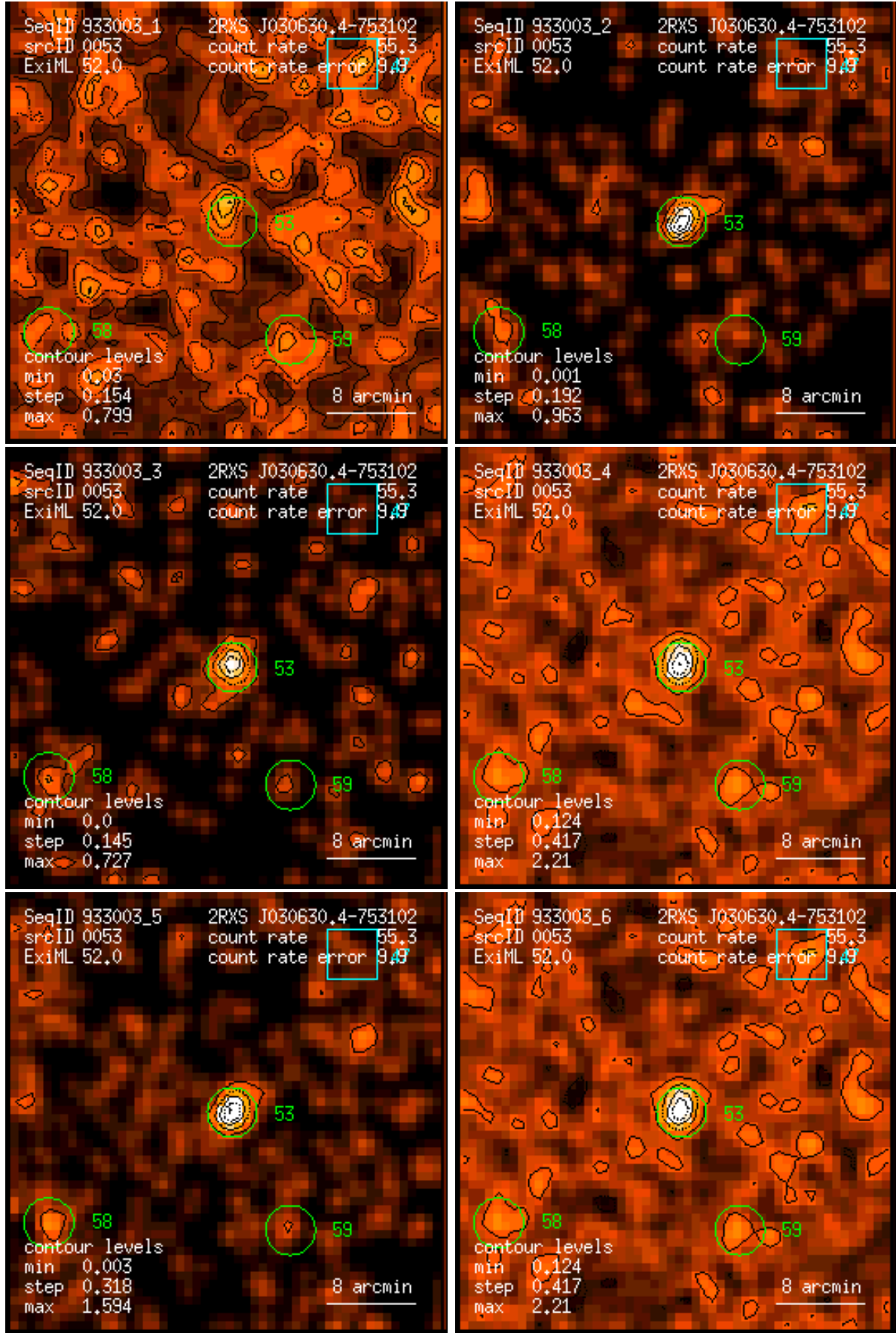
Figure 53: RASS 933003: detection 0053: band rate images, Gaussian filter: (1) PSPC channels 11 – 41, (2) 52 – 90, (3) 91 – 201, (4) 11 – 235, (5) 52 – 201, (6) 11 – 201. Broad band rates in counts/ks. Band rate contour levels in counts/ks/arcmin 2 .
