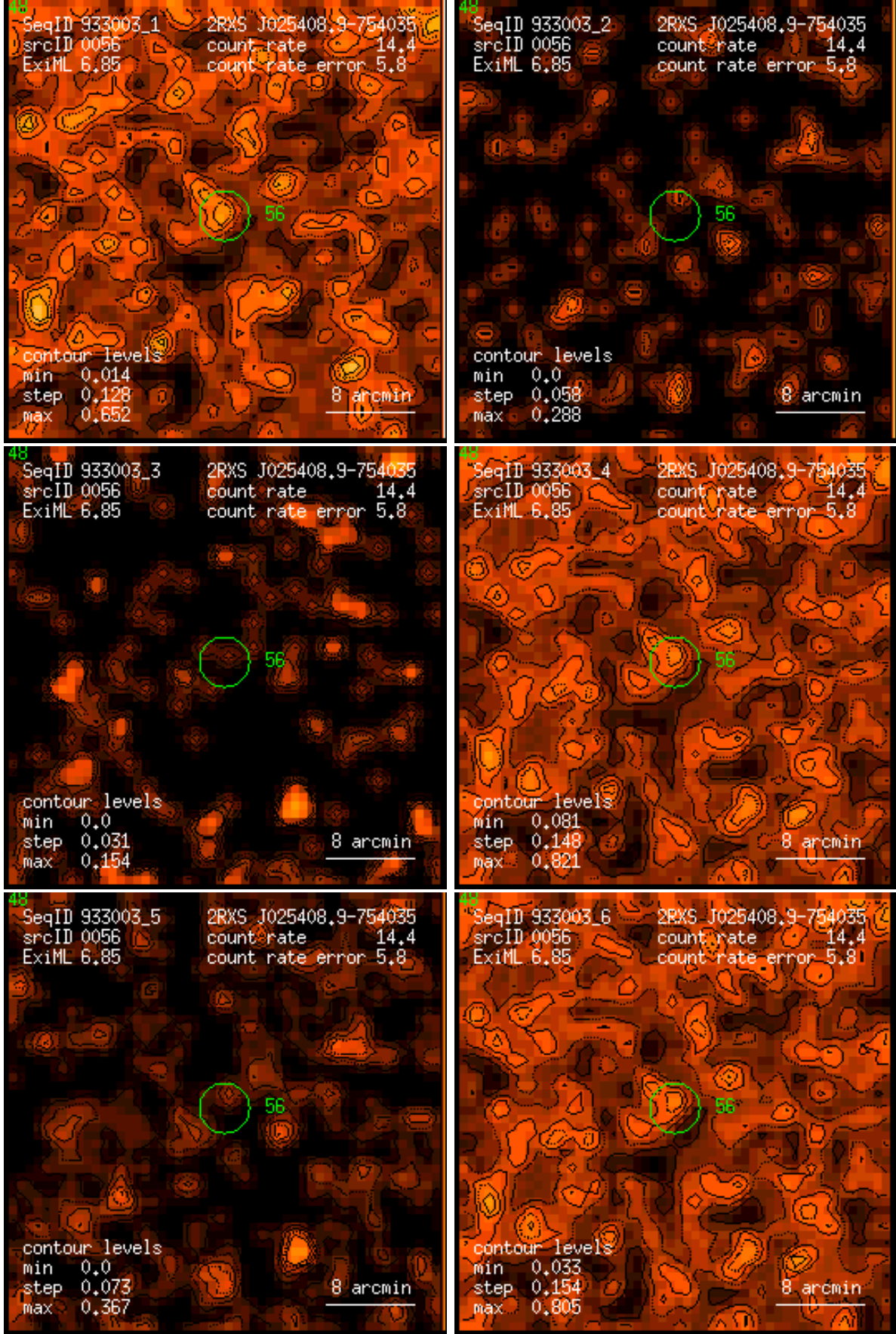
Figure 56: RASS 933003: detection 0056: band rate images, Gaussian filter: (1) PSPC channels 11 – 41, (2) 52 – 90, (3) 91 – 201, (4) 11 – 235, (5) 52 – 201, (6) 11 – 201. Broad band rates in counts/ks. Band rate contour levels in counts/ks/arcmin 2 .
