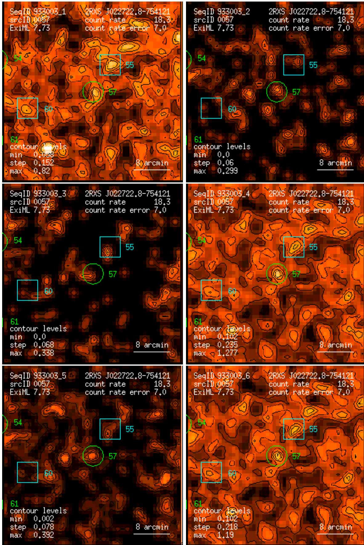
Figure 57: RASS 933003: detection 0057: band rate images, Gaussian filter: (1) PSPC channels 11 – 41, (2) 52 – 90, (3) 91 – 201, (4) 11 – 235, (5) 52 – 201, (6) 11 – 201. Broad band rates in counts/ks. Band rate contour levels in counts/ks/arcmin 2 .
