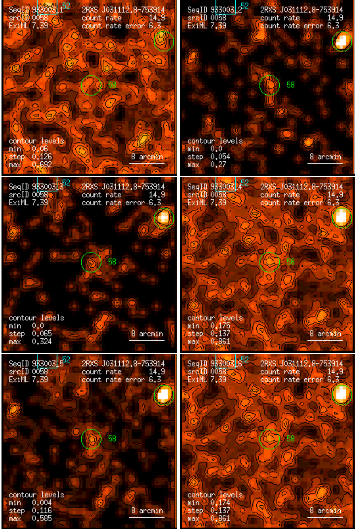
Figure 58: RASS 933003: detection 0058: band rate images, Gaussian filter: (1) PSPC channels 11 – 41, (2) 52 – 90, (3) 91 – 201, (4) 11 – 235, (5) 52 – 201, (6) 11 – 201. Broad band rates in counts/ks. Band rate contour levels in counts/ks/arcmin 2 .
