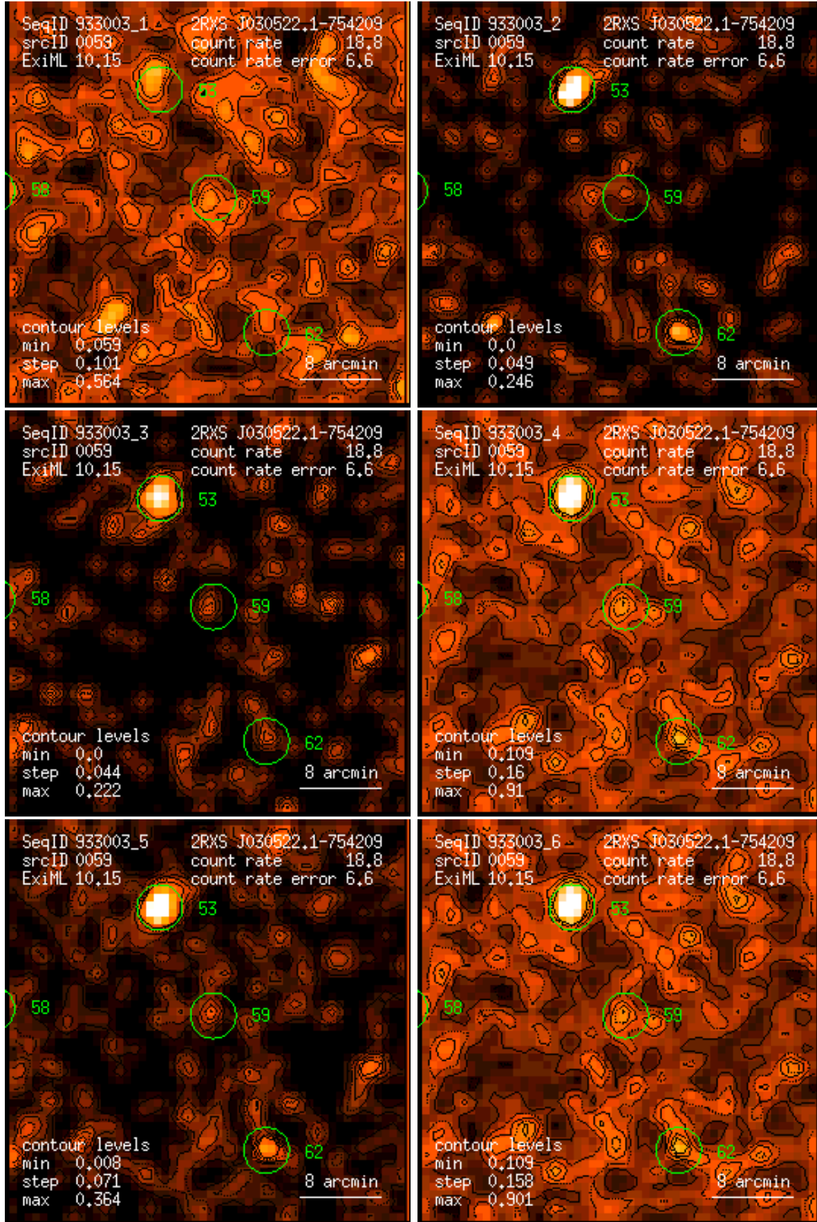
Figure 59: RASS 933003: detection 0059: band rate images, Gaussian filter: (1) PSPC channels 11 – 41, (2) 52 – 90, (3) 91 – 201, (4) 11 – 235, (5) 52 – 201, (6) 11 – 201. Broad band rates in counts/ks. Band rate contour levels in counts/ks/arcmin 2 .
