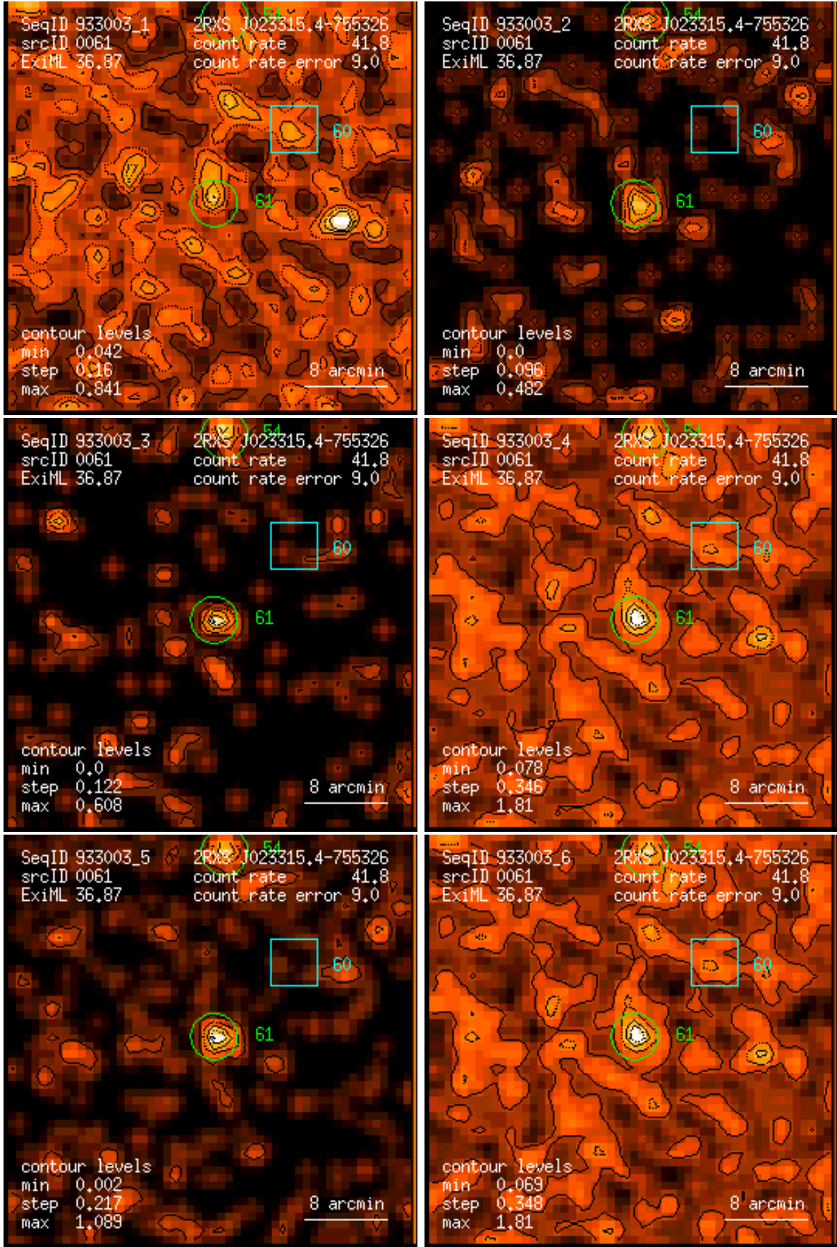
Figure 61: RASS 933003: detection 0061: band rate images, Gaussian filter: (1) PSPC channels 11 – 41, (2) 52 – 90, (3) 91 – 201, (4) 11 – 235, (5) 52 – 201, (6) 11 – 201. Broad band rates in counts/ks. Band rate contour levels in counts/ks/arcmin 2 .
