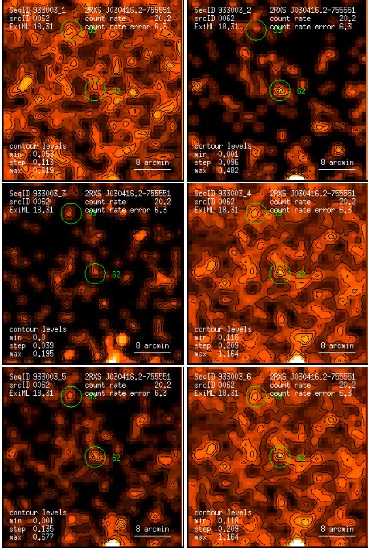
Figure 62: RASS 933003: detection 0062: band rate images, Gaussian filter: (1) PSPC channels 11 – 41, (2) 52 – 90, (3) 91 – 201, (4) 11 – 235, (5) 52 – 201, (6) 11 – 201. Broad band rates in counts/ks. Band rate contour levels in counts/ks/arcmin 2 .
