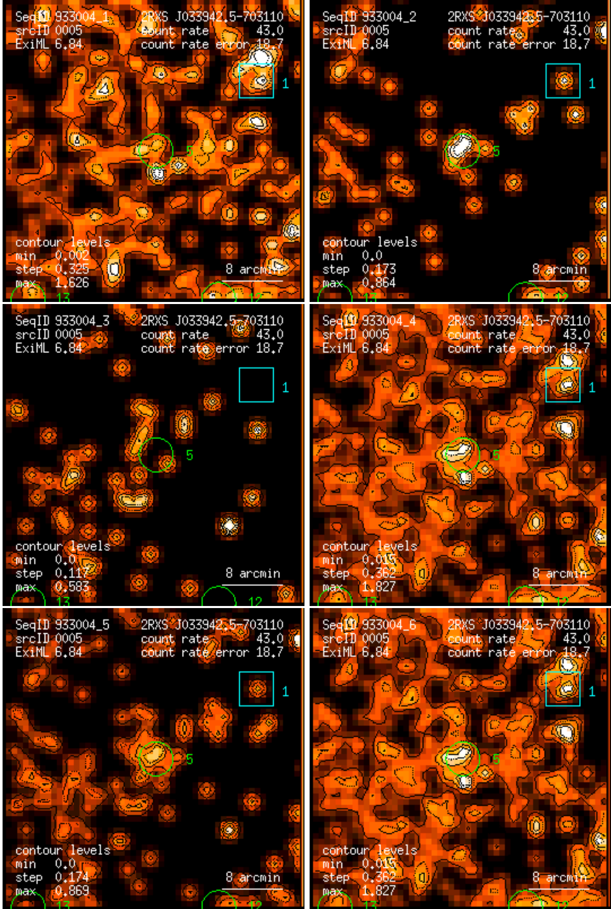
Figure 5: RASS 933004: detection 0005: band rate images, Gaussian filter: (1) PSPC channels 11 – 41, (2) 52 – 90, (3) 91 – 201, (4) 11 – 235, (5) 52 – 201, (6) 11 – 201. Broad band rates in counts/ks. Band rate contour levels in counts/ks/arcmin 2 .
