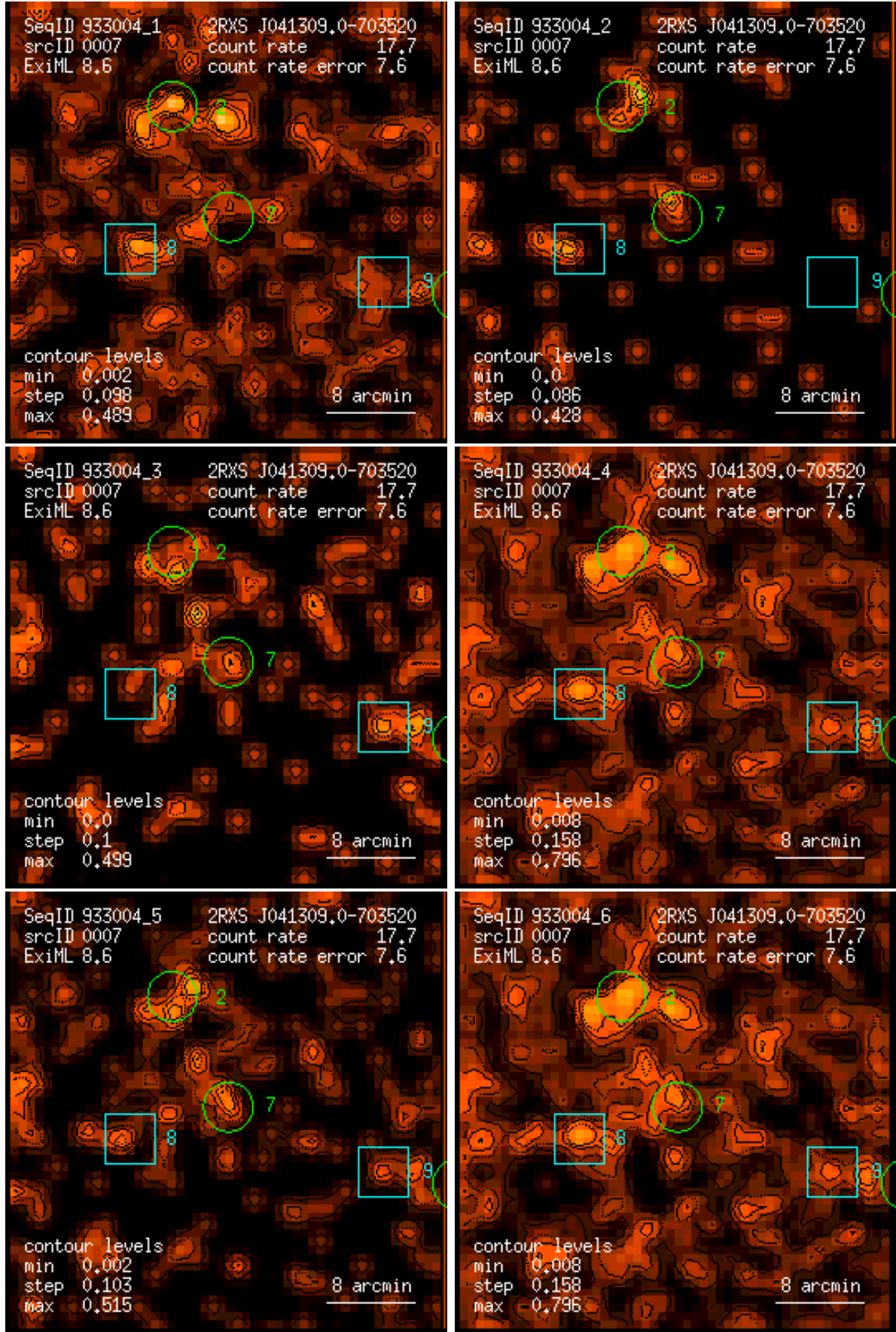
Figure 7: RASS 933004: detection 0007: band rate images, Gaussian filter: (1) PSPC channels 11 – 41, (2) 52 – 90, (3) 91 – 201, (4) 11 – 235, (5) 52 – 201, (6) 11 – 201. Broad band rates in counts/ks. Band rate contour levels in counts/ks/arcmin 2 .
