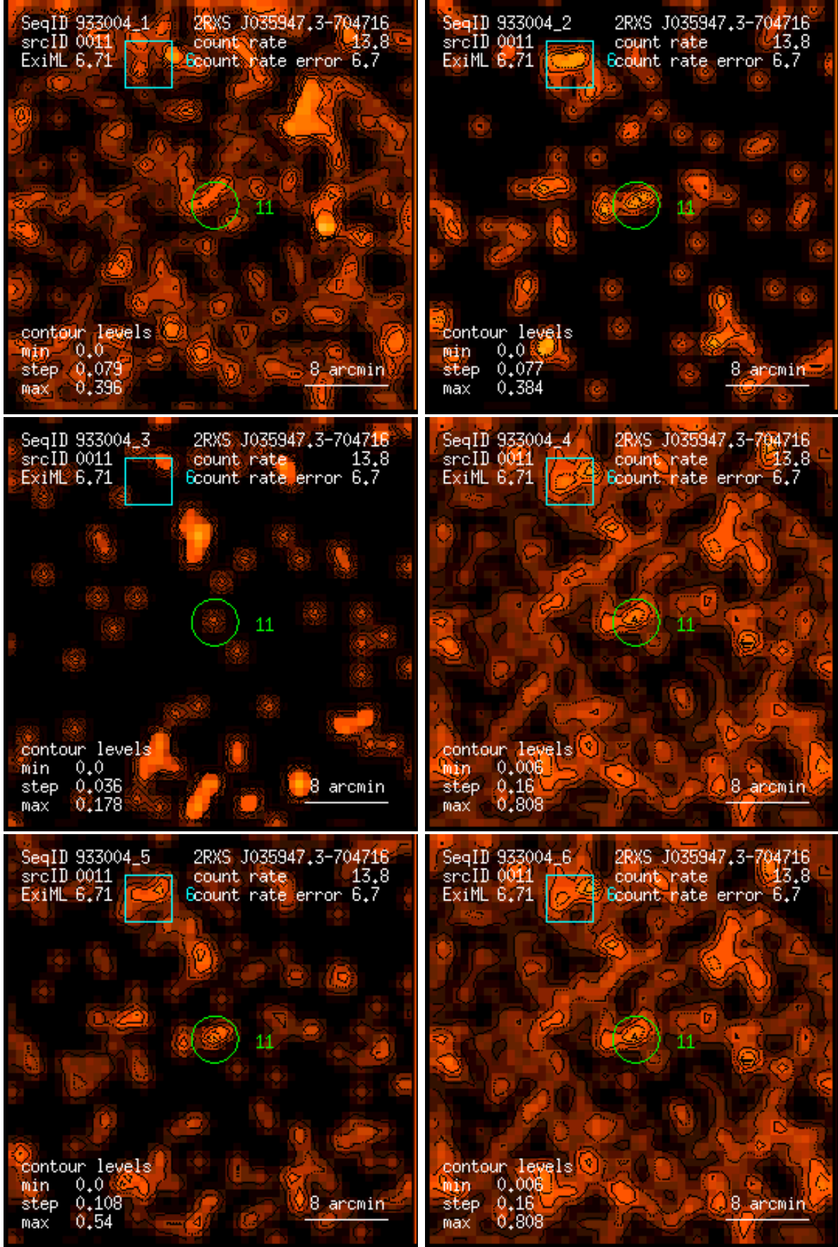
Figure 11: RASS 933004: detection 0011: band rate images, Gaussian filter: (1) PSPC channels 11 – 41, (2) 52 – 90, (3) 91 – 201, (4) 11 – 235, (5) 52 – 201, (6) 11 – 201. Broad band rates in counts/ks. Band rate contour levels in counts/ks/arcmin 2 .
