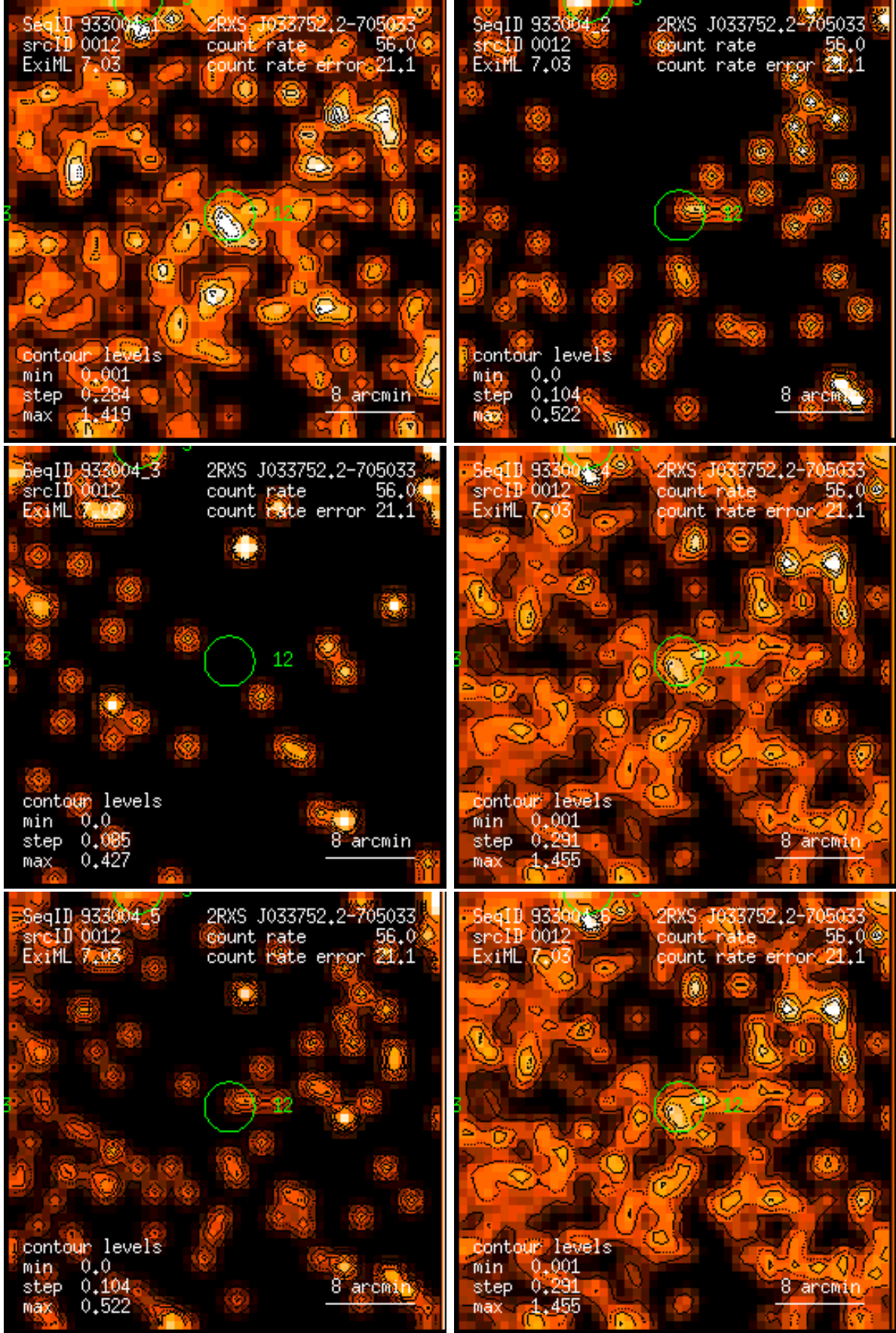
Figure 12: RASS 933004: detection 0012: band rate images, Gaussian filter: (1) PSPC channels 11 – 41, (2) 52 – 90, (3) 91 – 201, (4) 11 – 235, (5) 52 – 201, (6) 11 – 201. Broad band rates in counts/ks. Band rate contour levels in counts/ks/arcmin 2 .
