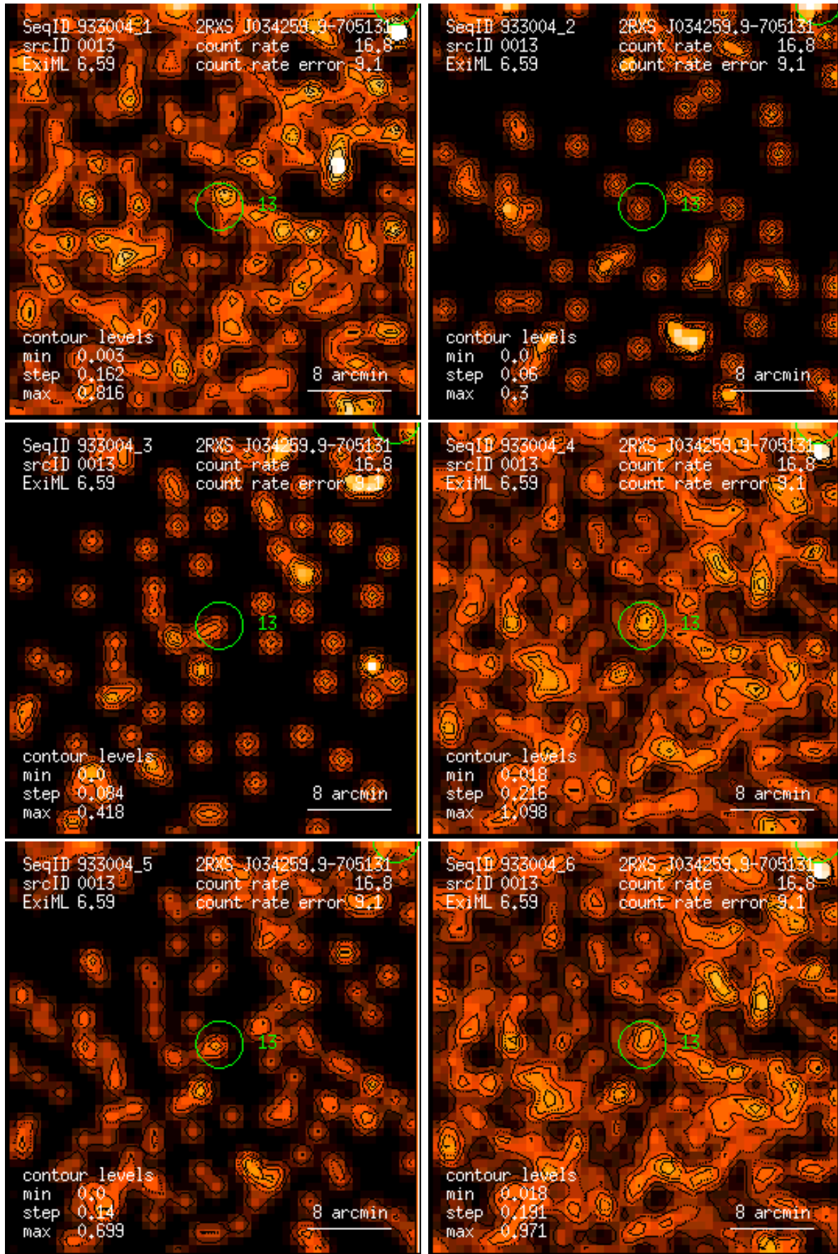
Figure 13: RASS 933004: detection 0013: band rate images, Gaussian filter: (1) PSPC channels 11 – 41, (2) 52 – 90, (3) 91 – 201, (4) 11 – 235, (5) 52 – 201, (6) 11 – 201. Broad band rates in counts/ks. Band rate contour levels in counts/ks/arcmin 2 .
