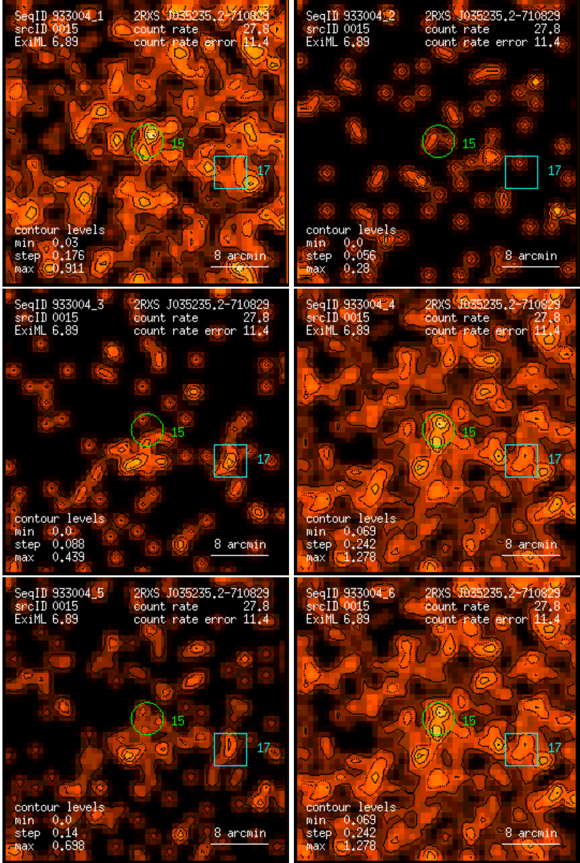
Figure 15: RASS 933004: detection 0015: band rate images, Gaussian filter: (1) PSPC channels 11 – 41, (2) 52 – 90, (3) 91 – 201, (4) 11 – 235, (5) 52 – 201, (6) 11 – 201. Broad band rates in counts/ks. Band rate contour levels in counts/ks/arcmin 2 .
