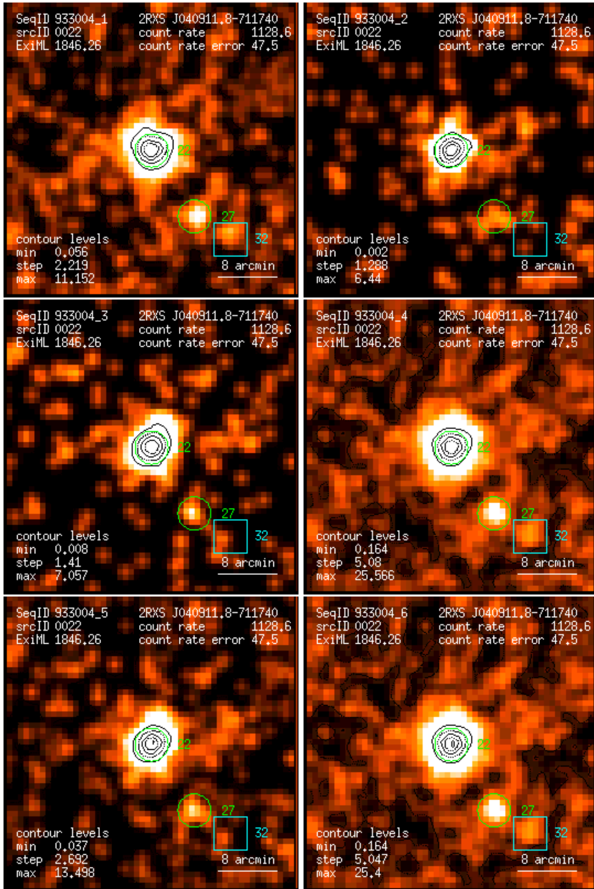
Figure 22: RASS 933004: detection 0022: band rate images, Gaussian filter: (1) PSPC channels 11 – 41, (2) 52 – 90, (3) 91 – 201, (4) 11 – 235, (5) 52 – 201, (6) 11 – 201. Broad band rates in counts/ks. Band rate contour levels in counts/ks/arcmin 2 .
