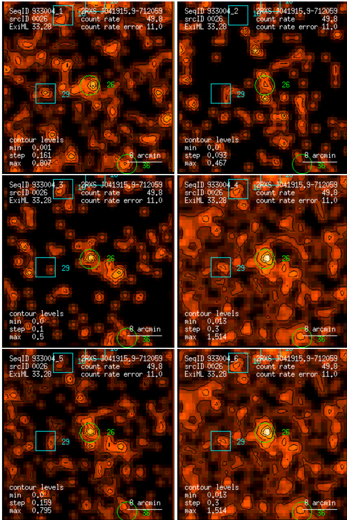
Figure 26: RASS 933004: detection 0026: band rate images, Gaussian filter: (1) PSPC channels 11 – 41, (2) 52 – 90, (3) 91 – 201, (4) 11 – 235, (5) 52 – 201, (6) 11 – 201. Broad band rates in counts/ks. Band rate contour levels in counts/ks/arcmin 2 .
