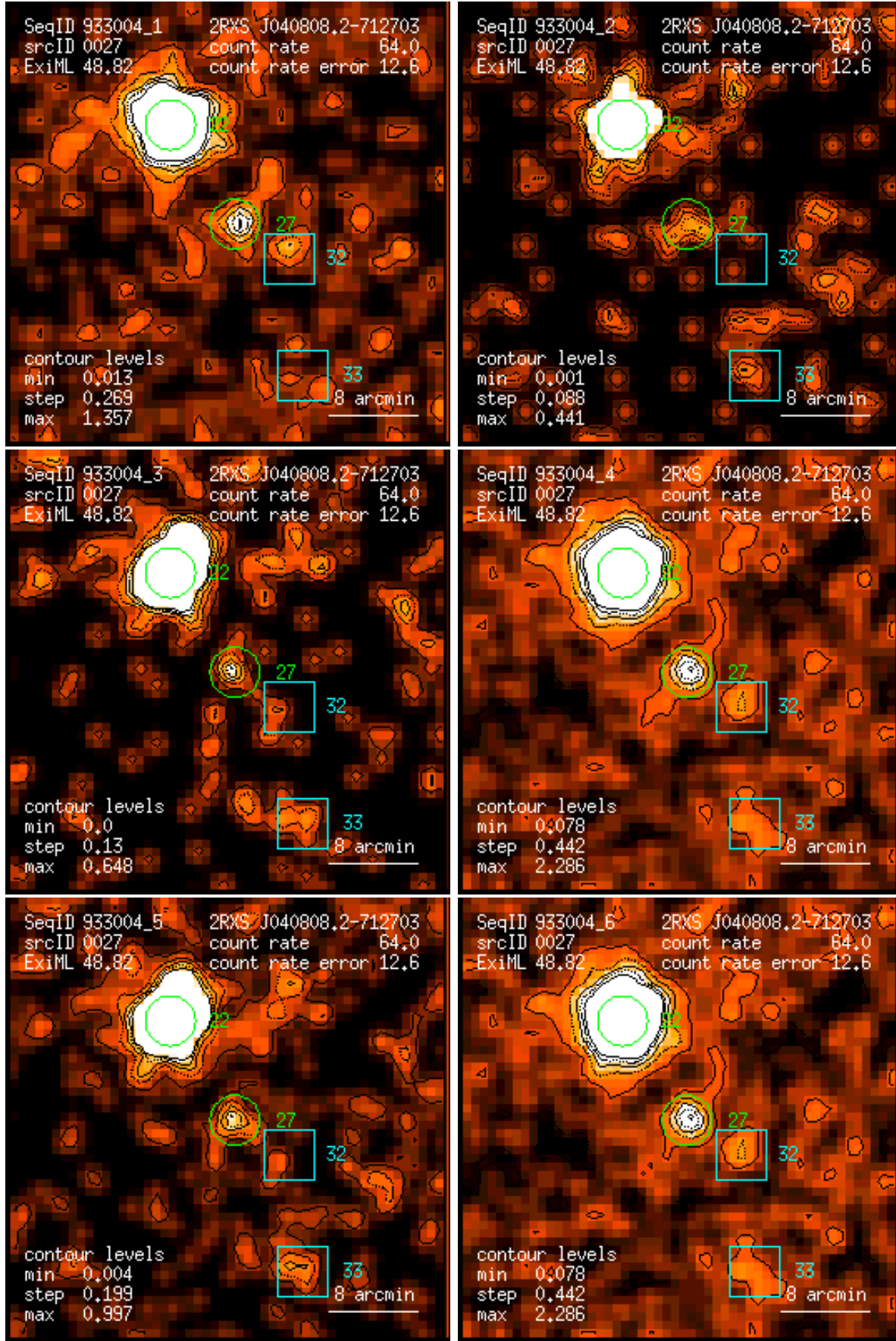
Figure 27: RASS 933004: detection 0027: band rate images, Gaussian filter: (1) PSPC channels 11 – 41, (2) 52 – 90, (3) 91 – 201, (4) 11 – 235, (5) 52 – 201, (6) 11 – 201. Broad band rates in counts/ks. Band rate contour levels in counts/ks/arcmin 2 .
