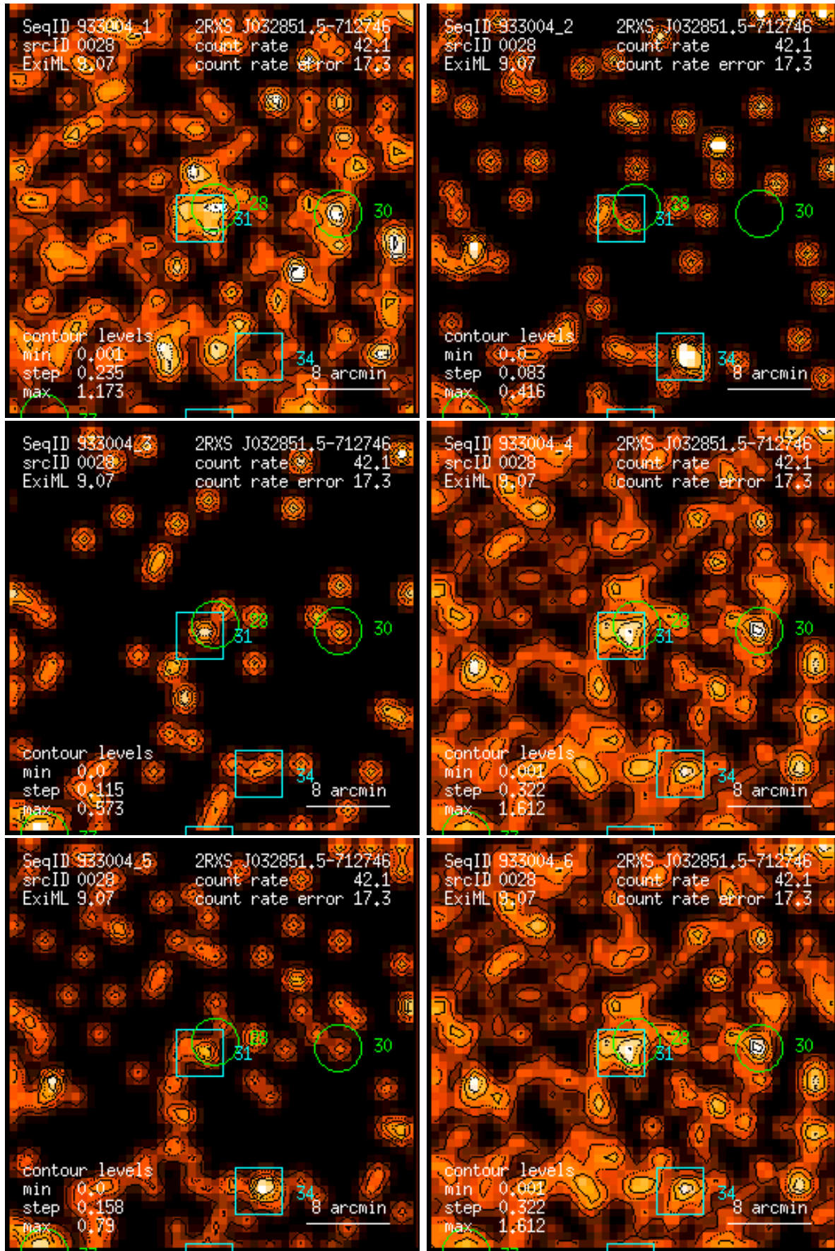
Figure 28: RASS 933004: detection 0028: band rate images, Gaussian filter: (1) PSPC channels 11 – 41, (2) 52 – 90, (3) 91 – 201, (4) 11 – 235, (5) 52 – 201, (6) 11 – 201. Broad band rates in counts/ks. Band rate contour levels in counts/ks/arcmin 2 .
