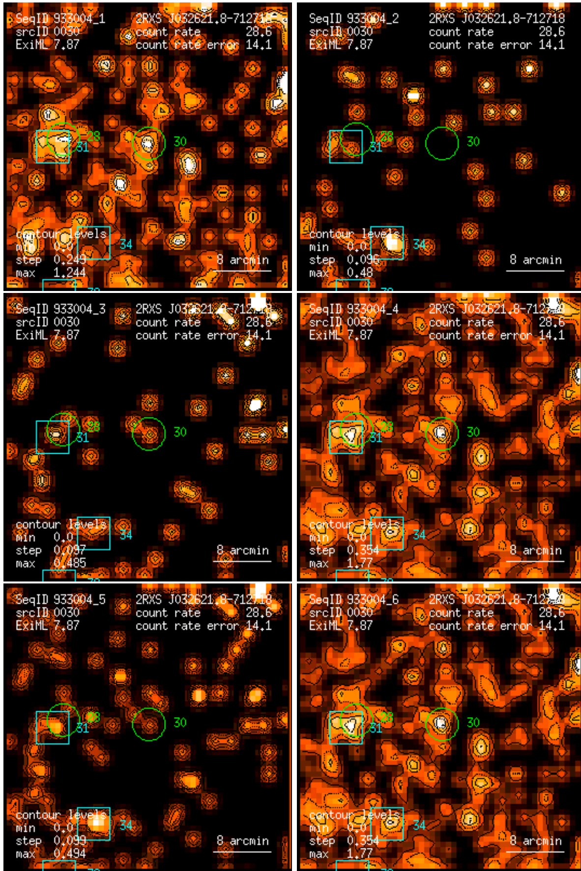
Figure 30: RASS 933004: detection 0030: band rate images, Gaussian filter: (1) PSPC channels 11 – 41, (2) 52 – 90, (3) 91 – 201, (4) 11 – 235, (5) 52 – 201, (6) 11 – 201. Broad band rates in counts/ks. Band rate contour levels in counts/ks/arcmin 2 .
