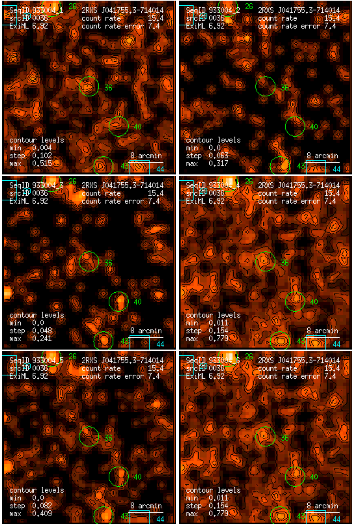
Figure 36: RASS 933004: detection 0036: band rate images, Gaussian filter: (1) PSPC channels 11 – 41, (2) 52 – 90, (3) 91 – 201, (4) 11 – 235, (5) 52 – 201, (6) 11 – 201. Broad band rates in counts/ks. Band rate contour levels in counts/ks/arcmin 2 .
